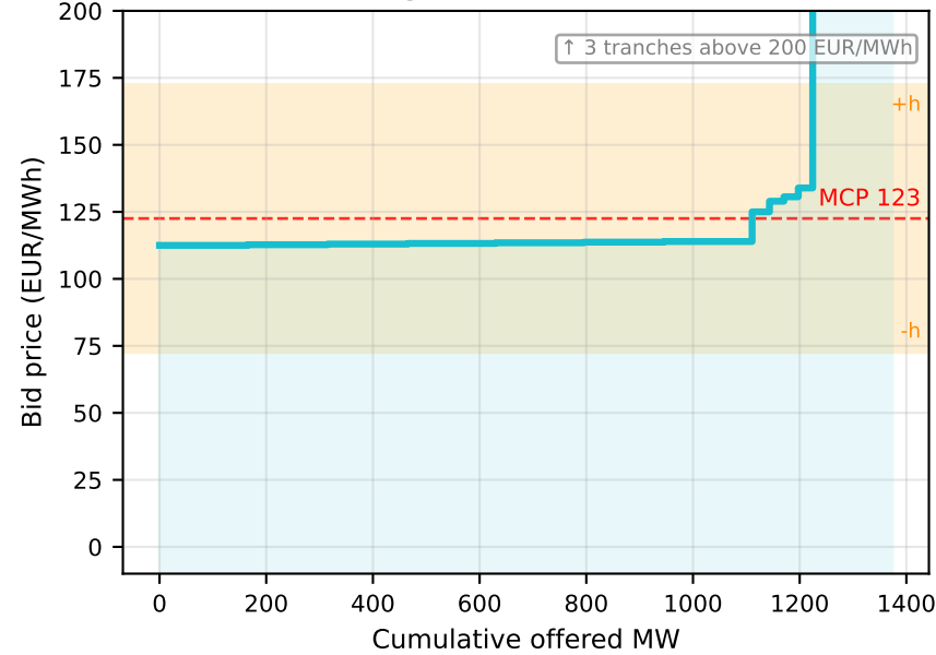
Pump-storage --- MUEL (14 tranches)
