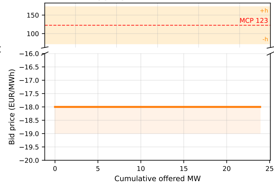
Solar PV (aggregator) --- EGVD503 (1 tranche)
