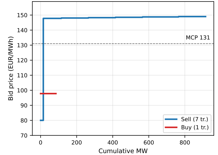
Solar PV (aggregator) --- GESTVD2 (S3 p17, 2024-11-01)
