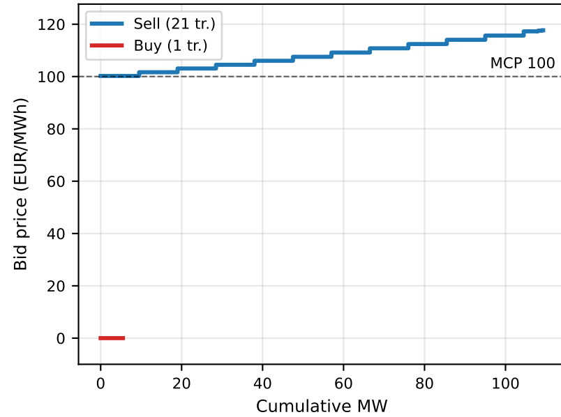
Nuclear --- COF1 (S2 p1, 2024-07-22)
