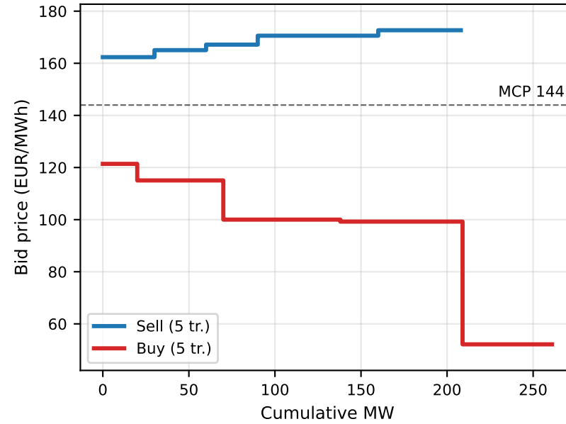
Solar PV (aggregator) --- GESTVD2 (S3 p17, 2024-11-01)
