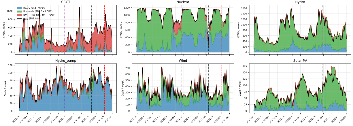
Figure 11: Weekly three-component decomposition of dispatch, by technology. PDBC (blue, day-ahead-cleared) + bilateral executions (green) + IDA + REE real-time top-up (red) = final post-IDA dispatch (black). Vertical guides: MTU15-IDA, April 2025 blackout, MTU15-DA.
