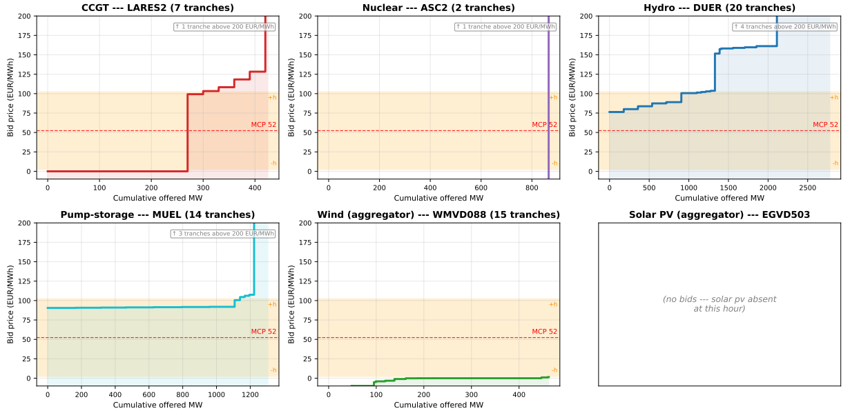
Figure 12: Representative day-ahead supply curves by technology, 2025-12-04 hour 01 quarter 4 (flat overnight hour on a windy night). Same colour scheme and broken y-axis convention as Figure 12. The wind panel (WMVD088) shows a 15-tranche aggregator micro-ladder concentrated in [-20, +1.5] EUR/MWh, well below the band.
