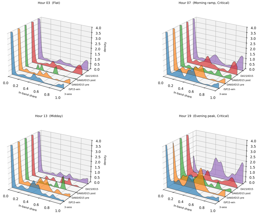
Hydro: in-band MW share distribution across regimes — sliced by hour-of-day
