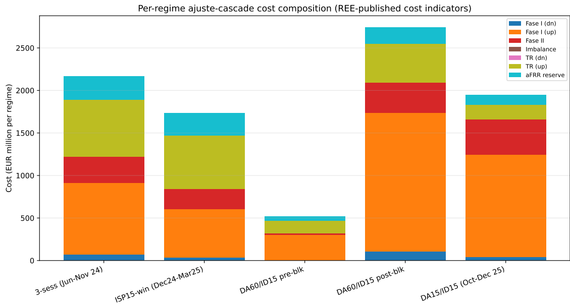
Figure 33: Stacked cost composition per regime. Bar height = total ajuste cost. Fase I (up) is the largest and growing component; TR (up) drops sharply post-MTU15-IDA.
