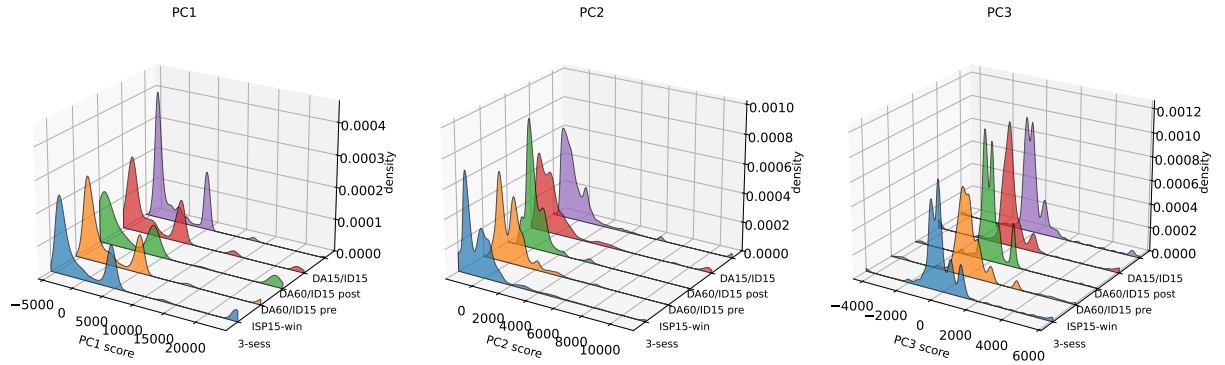
Figure 21: CCGT: distribution of functional-SA PC scores across regimes. Each panel is a 3D ridge plot of one principal component score; one curve per regime, stacked along the y -axis. Bimodality emerges post-MTU15-IDA on PC1 and PC2 (firms with cap-padded ladders vs firms bidding near MCP).
