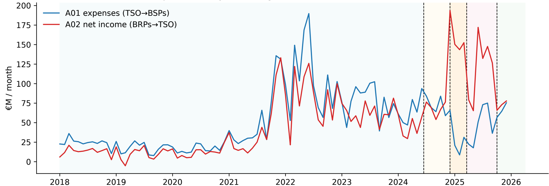
Spain monthly balancing financial balance (ENTSO-E A87)
