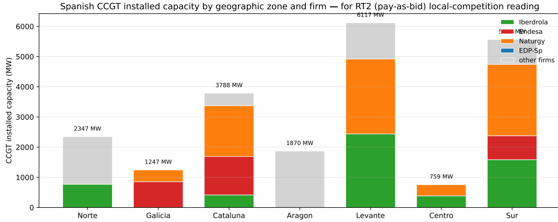
Figure 40: Spanish CCGT installed capacity (MW) by zone and firm. Bars stack each firm’s MW; zone labels (Sur, Levante, etc.) are grouped from plant-city assignments. Galicia and Centro are duopolies; Sur / Levante / Cataluña have wider firm diversity but GN holds the largest share in each.
