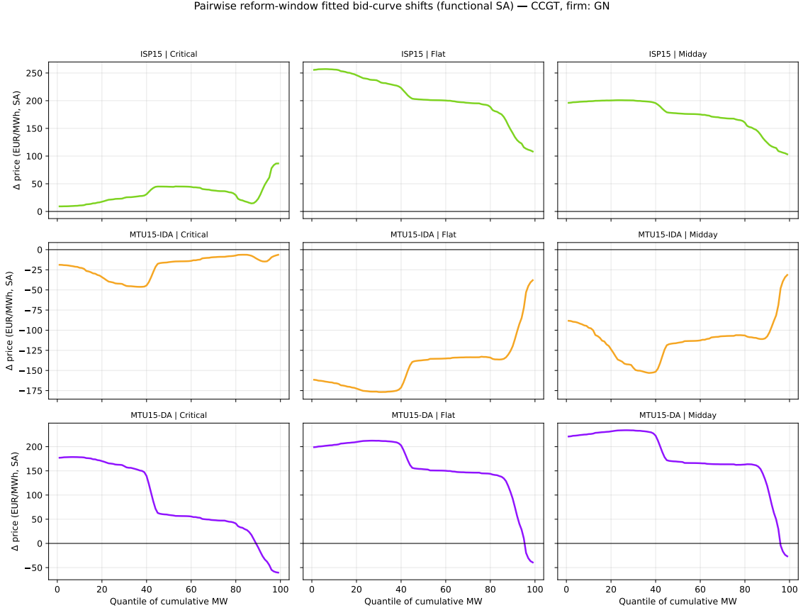
Figure 15: CCGT pairwise reform-window fitted bid-curve shifts on functionally-deseasonalised curves (firm: GN). Each row = a reform; each column = hour-class. The fitted shift is \sum_k \beta_k \phi_k(q) . Positive ordinate = bid curve shifts up under the reform.
