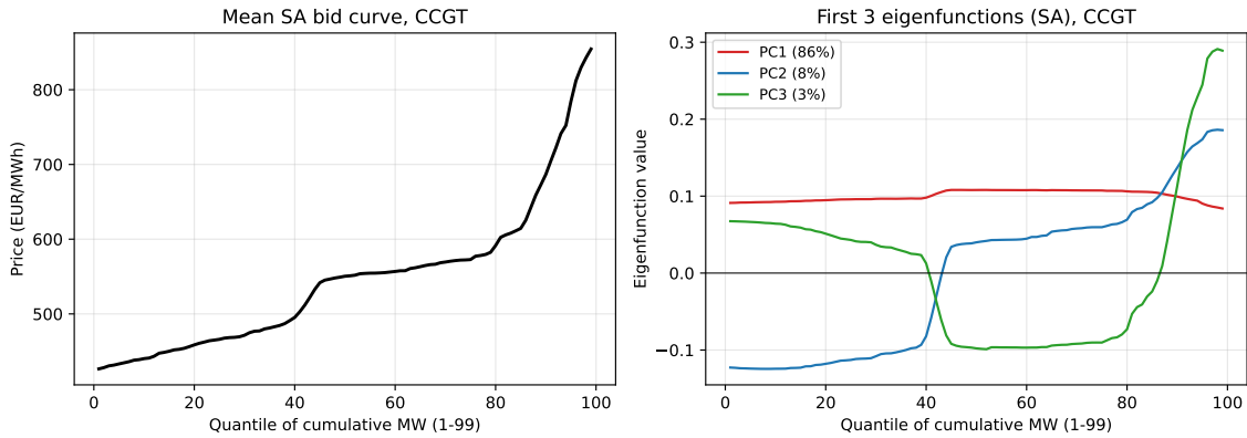
Figure 14: CCGT functional-SA bid-curve fPCA basis. Left: mean S^{-1}(q) across all CCGT (unit, date, period) deseasonalised cells. The familiar L-shape persists — functional SA strips the seasonal cycle but preserves the within-tech bid-stack geometry. Right: first 3 eigenfunctions. PC1 is essentially a uniform shift across all quantiles (level effect; 86% of curve variance). PC2 is a high-low region trade-off (8%, cheap vs scarcity tilt). PC3 (3%) is finer shape variation around the scarcity-mid transition. Raw-pipeline eigenfunctions are visually indistinguishable; the seasonal cycle was a small share of total curve variance even though it was material in EUR/MWh for individual reform-pairwise coefficients.
