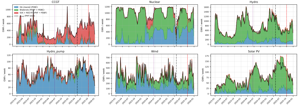
Figure 10: Weekly three-component decomposition of dispatch, by technology. PDBC (blue, day-ahead-cleared) + bilateral executions (PDBF – PDBC, green) + post-DA REE intervention layer (PHF – PDBF, red) = final post-IDA dispatch (black, equivalent to PHF). The red layer aggregates everything that happens to the schedule between the day-ahead programme (PDBF) and the post-IDA programme (PHF): Fase I pre-IDA up-redispatch and Fase II rebalance under PO 3.2 (paid pay-as-bid via the restriction-offer channel of PO 14.4 ap. 20.1, distinct from the day-ahead market offer), plus the net of all IDA clearings and REE’s post-IDA real-time technical-restrictions step. Within the red layer, Fase I dominates the post-blackout growth (Figure 4 and §6.3). Vertical guides: MTU15-IDA, April 2025 blackout, MTU15-DA.
