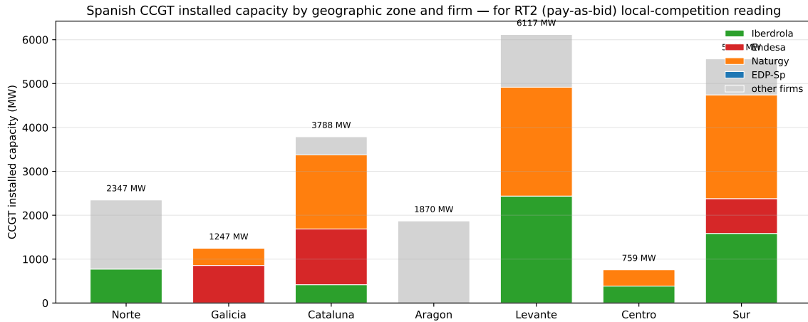
Figure 30: Spanish CCGT installed capacity (MW) by zone and firm. Bars stack each firm’s MW; zone labels (Sur, Levante, etc.) are grouped from plant-city assignments. Galicia and Centro are duopolies; Sur / Levante / Cataluña have wider firm diversity but GN holds the largest share in each.
