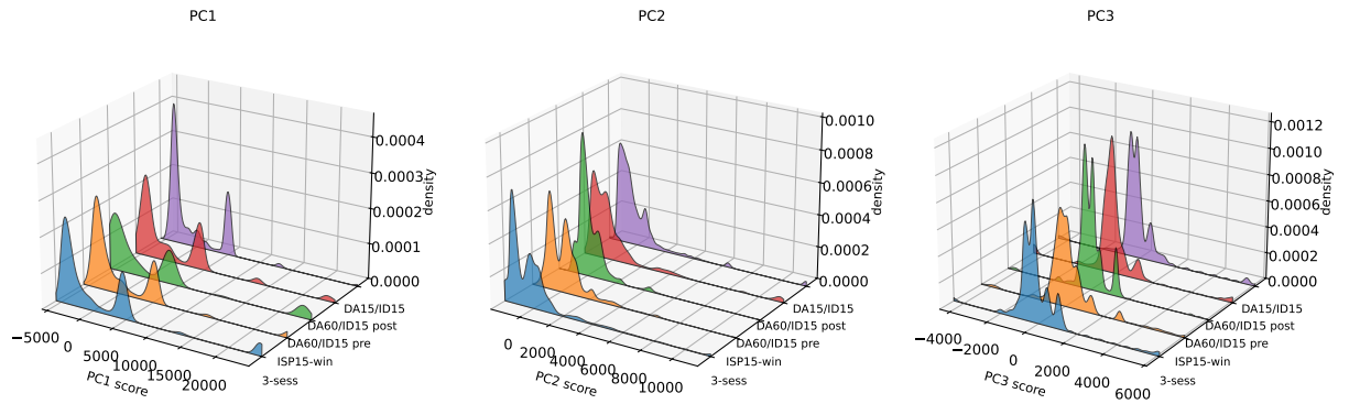
Figure 19: CCGT: distribution of functional-SA PC scores across regimes. Each panel is a 3D ridge plot of one principal component score; one curve per regime, stacked along the y -axis. Bimodality emerges post-MTU15-IDA on PC1 and PC2 (firms with cap-padded ladders vs firms bidding near MCP).
