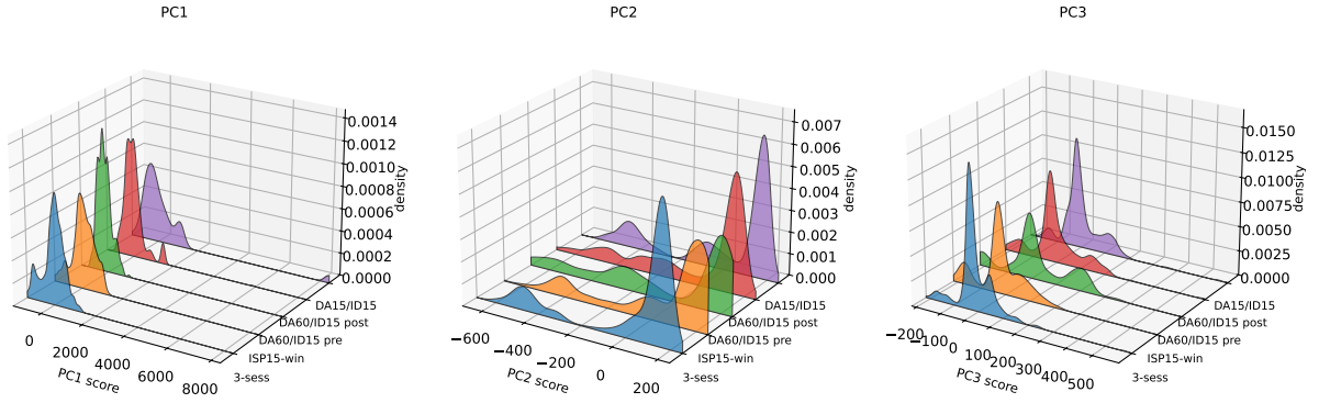
Figure 21: Hydro pump: distribution of functional-SA PC scores across regimes. Hydro_pump distributions are sharper than hydro (more concentrated PC1 mass), consistent with pumped storage's purer level-bidding posture.
