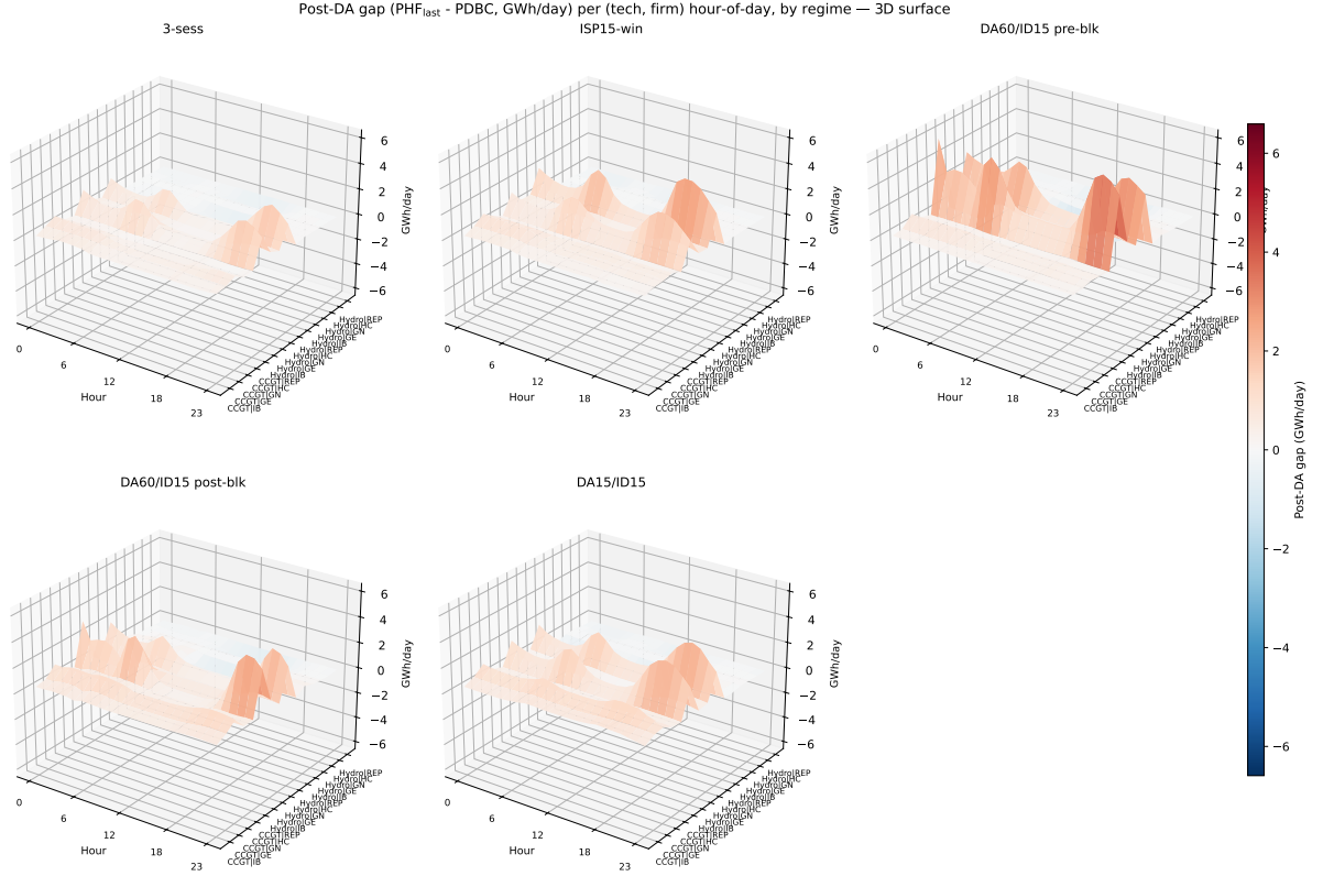
Figure 27: Post-DA gap ( \text{PHF}_{\text{last}} - \text{PDBC} , GWh/day) per (tech, firm) hour-of-day, by regime — 3D surface. x -axis: hour 0–23; y -axis: (tech, firm) row; z -axis: regime-mean post-DA gap (red = up, REE adds the unit; blue = down). Reform-window inclusion concentrates in critical hours for CCGT firms; the diurnal profile sharpens from 3-sess to DA15/ID15. Evening peak (18–22) is larger than morning ramp peak for IB/GN/HC CCGT. Heatmap version on disk ( post_da_gap_diurnal_heatmap.pdf ).
