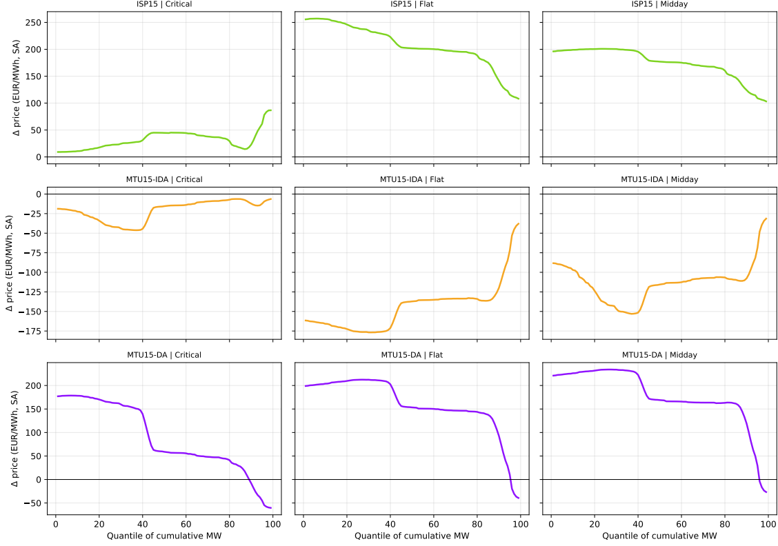
Figure 18: CCGT pairwise reform-window fitted bid-curve shifts on functionally-deseasonalised curves (firm: GN). Each row = a reform; each column = hour-class. The fitted shift is \sum_k \beta_k \phi_k(q) . Positive ordinate = bid curve shifts up under the reform.
