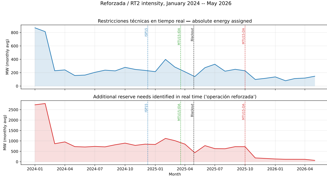
Figure 3: Reforzada / RT2 intensity, January 2024 – May 2026. Top panel: monthly average of absolute energy assigned via real-time technical restrictions (ESIOS indicator 10052). Bottom panel: monthly average of additional reserve needs identified in real time (ESIOS indicator 1880; coverage from 2021-05). Dashed vertical lines mark, in order, ISP15 (2024-12-09), MTU15-IDA (2025-03-19), the Iberian blackout (2025-04-28) and MTU15-DA (2025-10-01).
