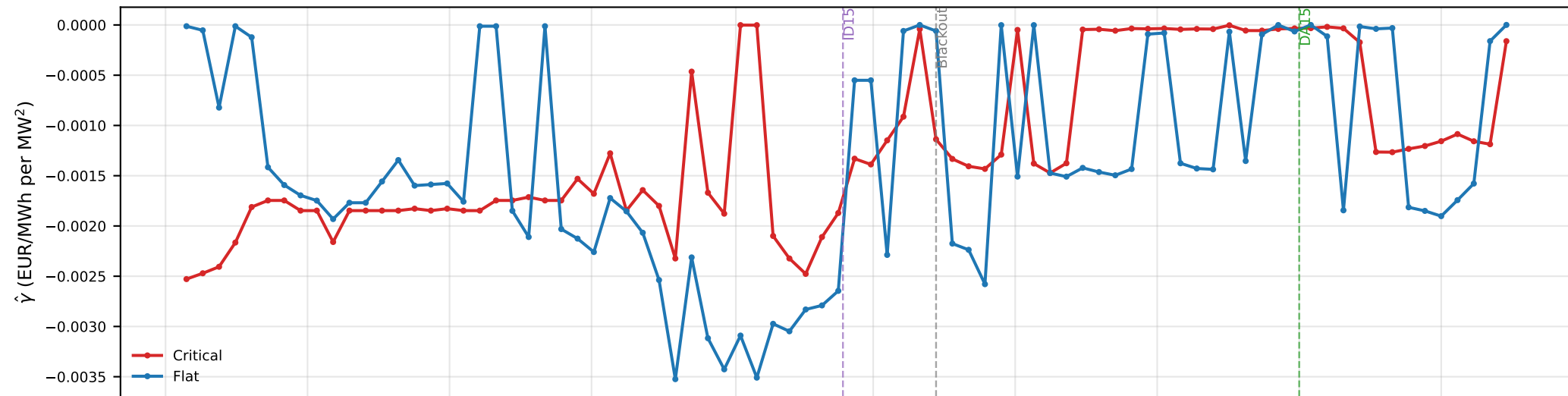
CCGT day-ahead per-curve gamma (critical = ramp hours, flat = overnight)
