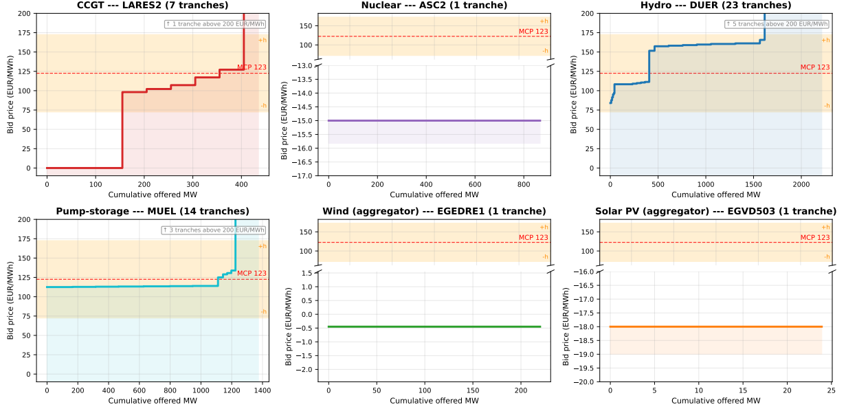
Figure 11: Representative day-ahead supply curves by technology, 2025-12-17 hour 17 quarter 4 (post-MTU15-DA, evening-ramp critical hour). Red dashed: MCP; orange band: in-band region [MCP \pm \delta] with \delta = 50 (§4.3). Panels with bid ranges far below the band use a broken y-axis for readability.
