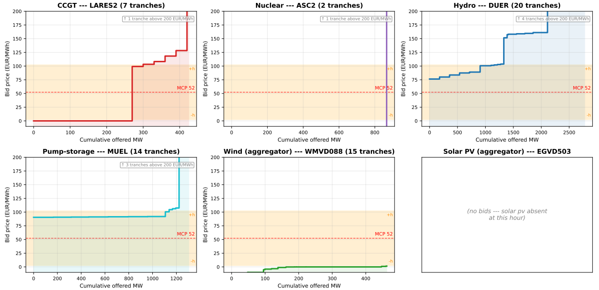
Figure 12: Representative day-ahead supply curves by technology, 2025-12-04 hour 01 quarter 4 (flat overnight hour on a windy night). Same colour scheme and broken y-axis convention as Figure 11. The wind panel (WMVD088) shows a 15-tranche aggregator micro-ladder concentrated in [-20, +1.5] EUR/MWh, well below the band.
