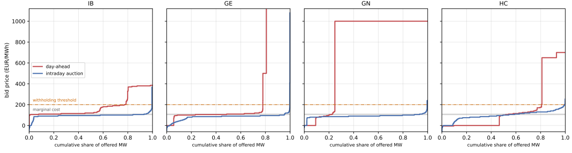
Figure 3: CCGT bid curves: day-ahead vs intraday auction, by firm (DA15/ID15). Each Big-4 CCGT fleet’s sell tranches aggregated into a supply curve (bid price vs cumulative share of offered MW). Grey band: bottom-up CCGT marginal cost; dash-dot line: the \sim 200 EUR/MWh withholding threshold. The day-ahead curve (red) carries the withholding shelf; the intraday-auction curve (blue) sits on the marginal-cost band for the whole book. Same units, same days — the withholding is a day-ahead-only strategy.
