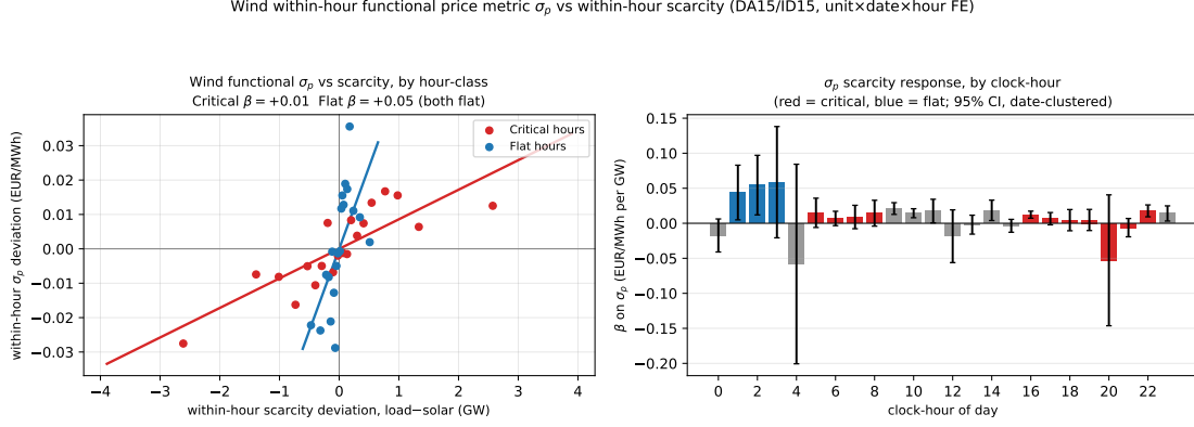
Figure 6: The wind functional price metric \sigma_p does not respond to within-hour scarcity (DA15/ID15, unit \times date \times hour fixed effects; band centred on the clock-hour-mean clearing price). Left: binned within-hour-demeaned \sigma_p against the within-hour-demeaned scarcity proxy (load minus solar forecast, GW), for critical and flat hours — both slopes essentially flat. Right: the slope for each clock-hour of the day (red = critical, blue = flat hours; date-clustered 95% intervals) — no hour reaches an economically meaningful response.
