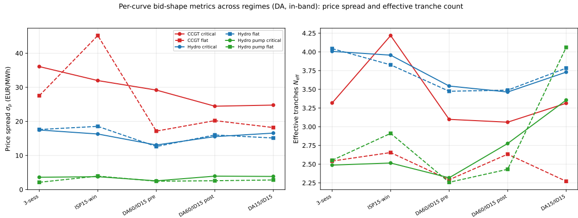
Figure 5: Per-curve bid-shape metrics across regimes (DA, in-band, data-driven band |p - \text{MCP}| \leq 140 ). Left: price spread \sigma_p ; right: effective tranche count N_{\text{eff}} . Each line is a (tech, hour-class) cell; solid = critical hours, dashed = flat. CCGT carries the widest price spread ( \sigma_p \approx 25\text{--}40 EUR/MWh) and it is larger in critical than flat hours in four of the five regimes — the strategic signal; Hydro is intermediate ( \sim 13\text{--}18 ) and Hydro pump near-flat ( \sim 3\text{--}4 ). N_{\text{eff}} sits at \sim 3\text{--}4 for the price-setting techs.
