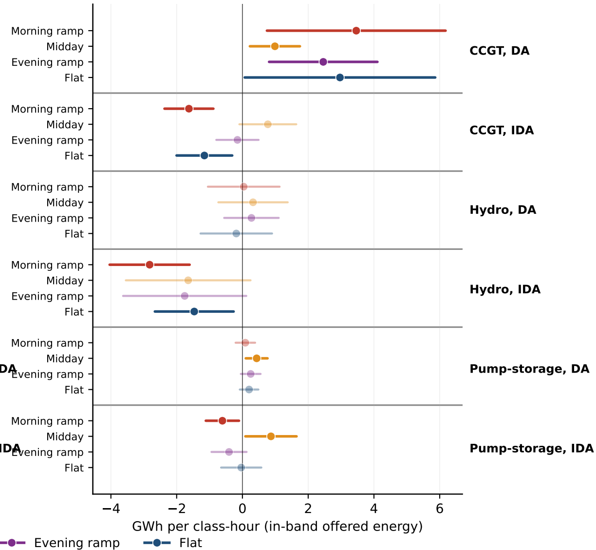
DA15 -- placebo-net level on in-band offered energy
