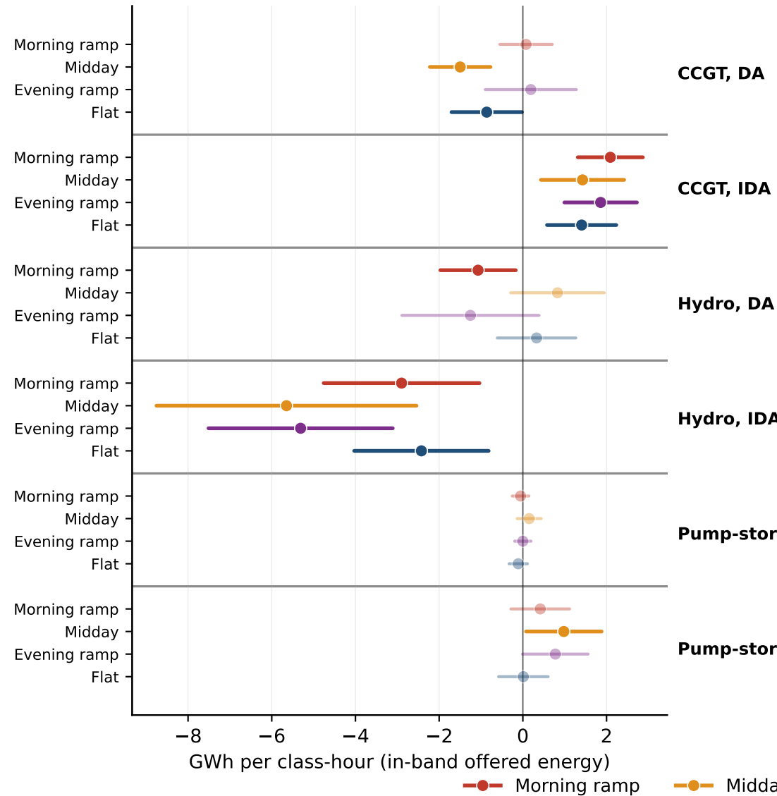
ID15 -- placebo-net level on in-band offered energy
