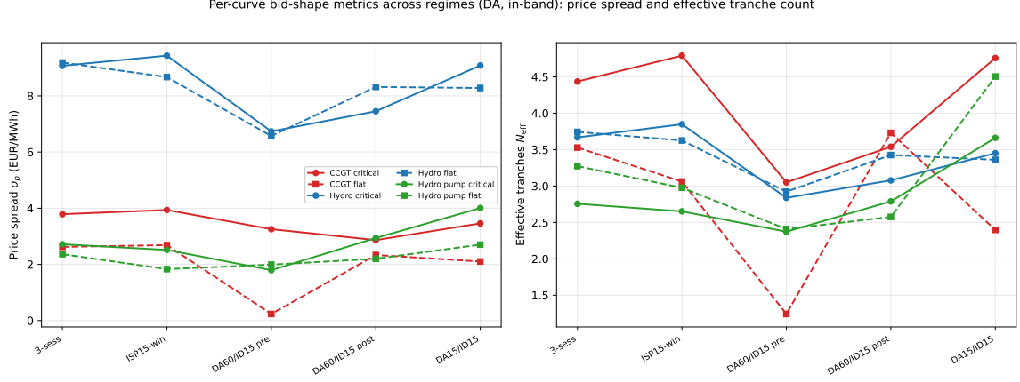
Figure 8: Per-curve bid-shape metrics across regimes (DA, in-band). Left: price spread \sigma_p ; right: effective tranche count N_{\text{eff}} . Each line is a (tech, hour-class) cell; solid = critical hours, dashed = flat. Hydro carries the widest price spread (water-value bidding spans a range); CCGT’s \sigma_p is consistently larger in critical than flat hours — the strategic signal. N_{\text{eff}} rises across the reform sequence for all three price-setting techs.
