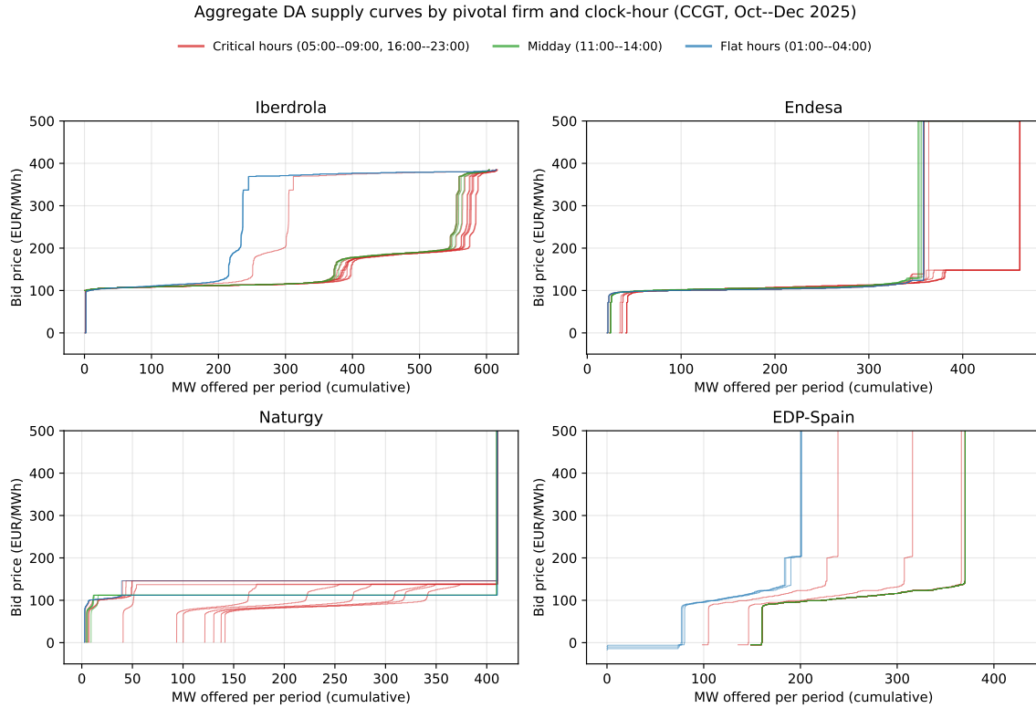
Figure 4: Aggregate DA supply curves by pivotal firm and clock-hour, CCGT, October–December 2025. One curve per (firm, clock-hour). Each curve is built per the EUPHEMIA aggregation rule (public description, sec. 7.1): pool all sell tranches across days for that (firm, hour), sort by ascending price, cumulate, and normalise by the number of (date, unit, period) cells. Red: each of the 11 critical hours. Green: each of the 4 midday hours (11:00–14:00, dropped from the DiD). Blue: each of the 3 flat hours. The same construction applied to Hydro, Wind, and Solar PV is in Appendix A.9.
