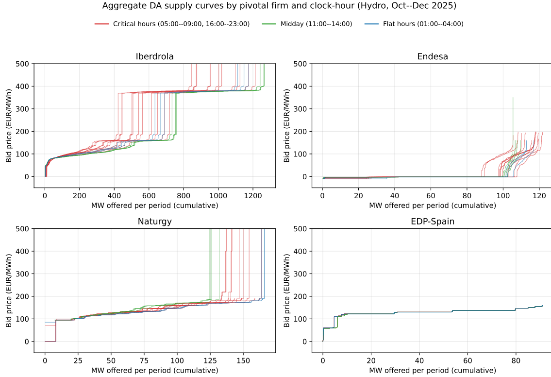
Figure 7: Aggregate DA supply curves, Hydro, October–December 2025. Same construction as Figure 4.
