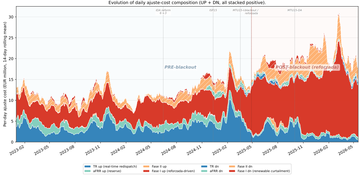
Figure 7: Daily adjustment-cost composition, 2023–2026 (EUR M / day, 14-day rolling mean). Each channel is the daily sum of the pay-as-bid system-cost series REE publishes via ESIOS: TR up/dn is real-time technical restrictions under PO 3.7 (cost of energy REE buys/sells to enforce grid security between gate closure and delivery); aFRR up/dn is the automatic Frequency Restoration Reserve energy cost; Fase I up/dn is the pre-IDA technical-restrictions process applied to PDBF (pay-as-bid of a separate restriction offer per PO 3.2 and PO 14.4 ap. 20.1, distinct from the day-ahead market offer); Fase II up/dn is the post-Fase-I rebalance that re-absorbs the up-redispatch into the schedule. All series are EUR sums collected at native 15-min granularity (raw daily totals smoothed only by the 14-day moving average), with down-direction channels taken as absolute values so the chart reads as gross costs REE pays providers in both directions. Up-direction stacked solid (TR-up, aFRR-up, Fase II up, Fase I up); down-direction stacked hatched. Blue background: pre-blackout (granularity reforms shrink the up-direction TR and aFRR channels through the ISP15-win and MTU15-IDA cutovers, visible against the stable 2023 baseline). Red background: post-blackout reforzada (Fase I up-redispatch balloons by EUR ~5 M/day, almost entirely CCGT voltage support; this is the level shift between the 2023 baseline and 2025-Q4 totals).
