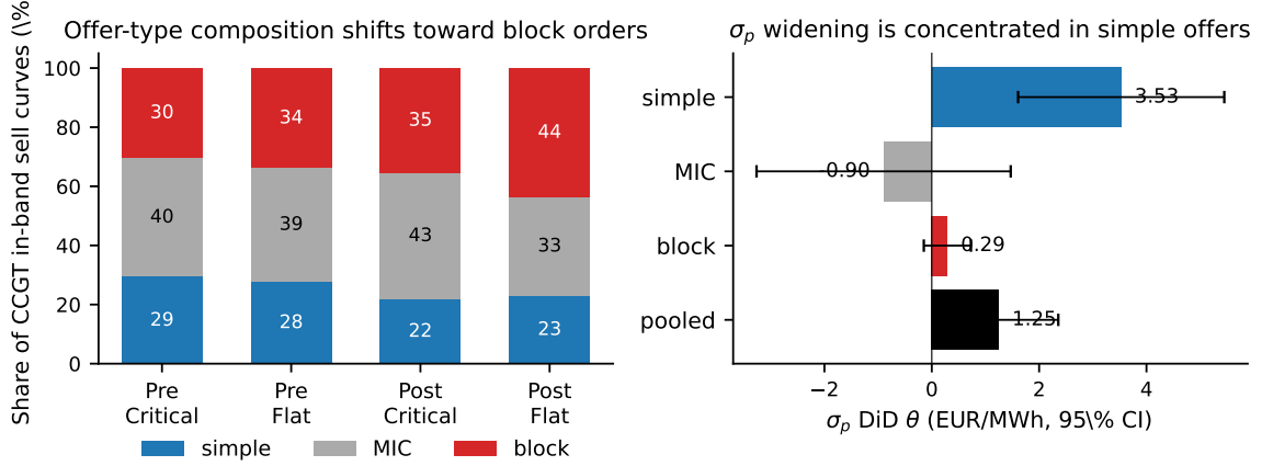
Figure 10: CCGT offer-type composition and within-type bid-shape DiD at DA15. Left: CCGT in-band sell-curve composition, pre vs post. Right: \sigma_p DiD by offer type, 95% CI. The HHI p DiD is negative within every type, so the deconcentration is not a composition artefact.
