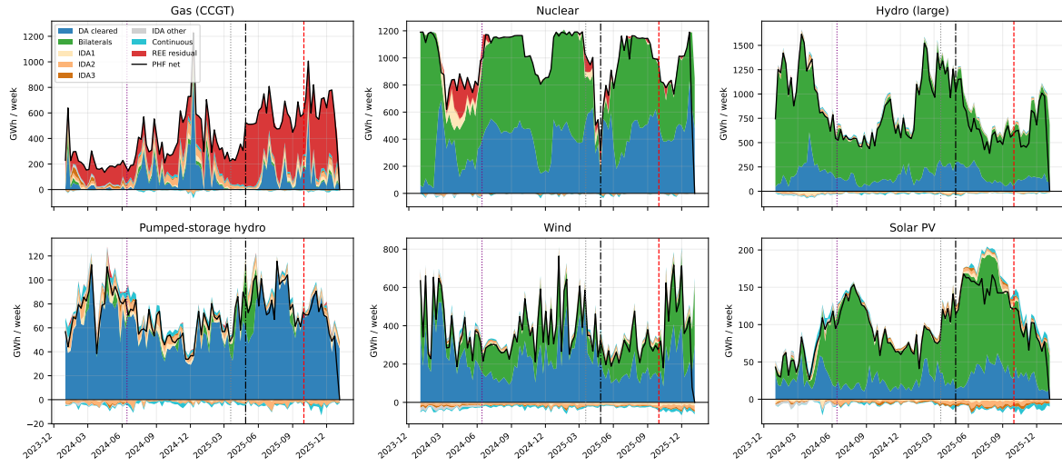
Figure 13: Weekly program cascade by technology. Chronological stack: day-ahead + bilaterals + IDA1–3 + continuous + post-IDA redispach; supply above zero, consumption and down-redispach below; black line = PHF net. Vertical guides: ID15, blackout, DA15.
