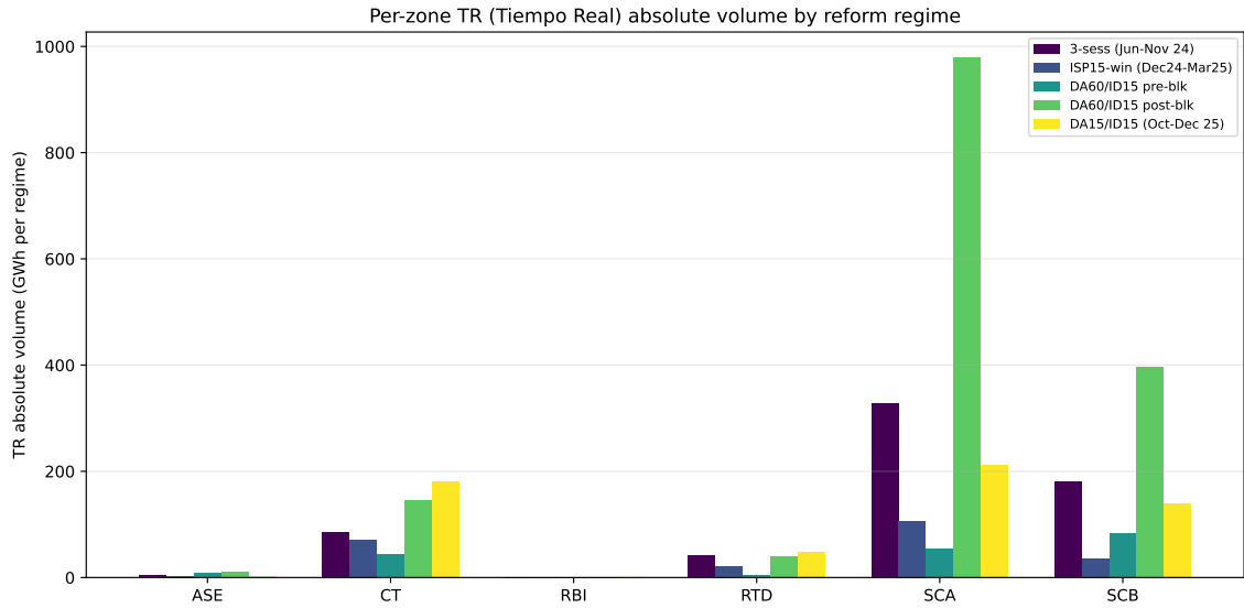
Figure 24: Per-zone TR volume by regime. The SCA/SCB spike in DA60/ID15 post-blk is the geographic footprint of operación reforzada (central + southern transmission constraints). CT zone TR stays consistently elevated.
