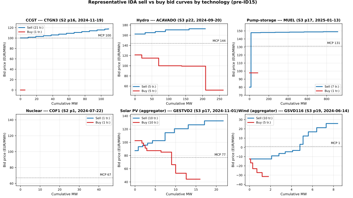
Figure 13: Representative IDA sell vs buy bid curves by technology, pre-ID15. One representative (unit, date, session, period) per tech. Blue: sell curve (supply, ascending in price). Red: buy curve (demand, descending in price). Dashed: MCP. Pre-ID15 window 2024-06-14 to 2025-03-18.
