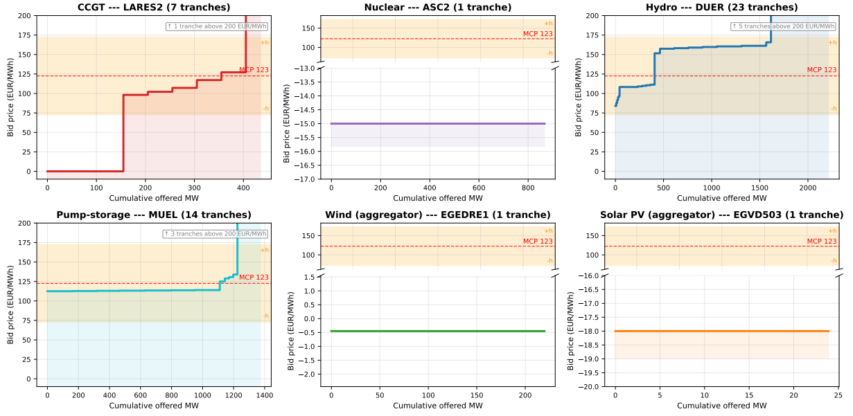
Figure 11: Representative day-ahead supply curves by technology, 2025-12-17 hour 17 quarter 4 (post-MTU15-DA, evening-ramp critical hour). Red dashed: MCP; orange band: in-band region [MCP \pm \delta] with \delta = 50 (§4.3). Panels with bid ranges far below the band use a broken y-axis for readability.
