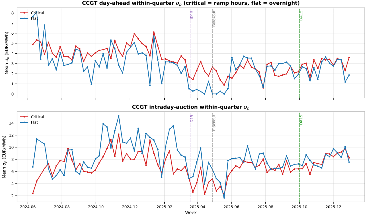
Figure 8: Weekly CCGT within-quarter \sigma_p by hour-class, 2024-06 to 2025-12. Top: day-ahead; Bottom: intraday-auction (latest-session in-band tranches, |p_k - MCP| \leq 50 EUR/MWh). Red: critical hours; blue: flat hours. Vertical dashes: ID15 (2025-03-19), blackout (2025-04-28), DA15 (2025-10-01).
