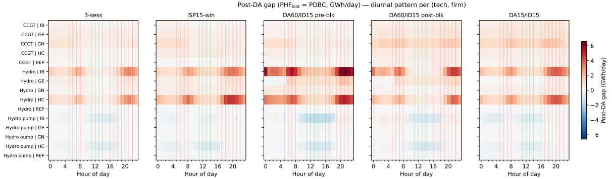
Figure 23: Post-DA gap ( \text{PHF}_{\text{last}} - \text{PDBC} , GWh/day) per (tech, firm) hour-of-day, by regime. Rows: (tech, firm); columns: hours 0–23; colour: regime-mean post-DA gap GWh/day at that cell (red = up, REE adds the unit; blue = down). Reform-window inclusion concentrates in critical hours (red vertical lines) for CCGT firms; the diurnal profile sharpens from 3-sess to DA15/ID15. Evening peak (18–22) is larger than morning ramp peak for IB/GN/HC CCGT.
