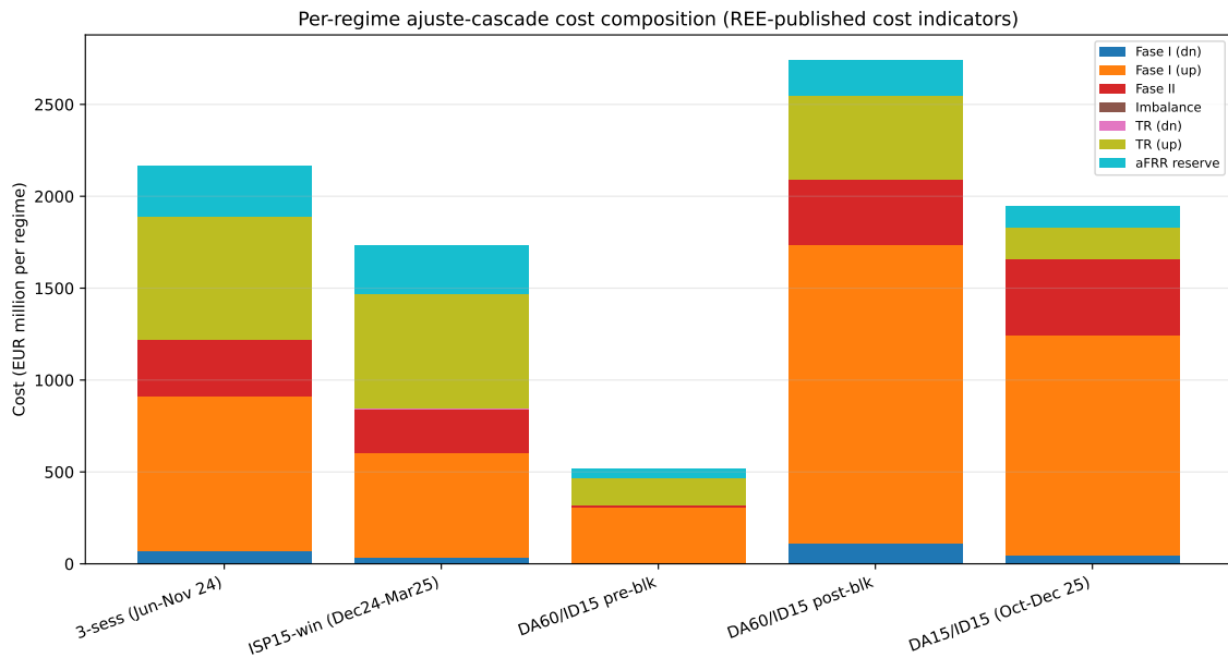
Figure 26: Stacked cost composition per regime. Bar height = total ajuste cost. Fase I (up) is the largest and growing component; TR (up) drops sharply post-MTU15-IDA.
