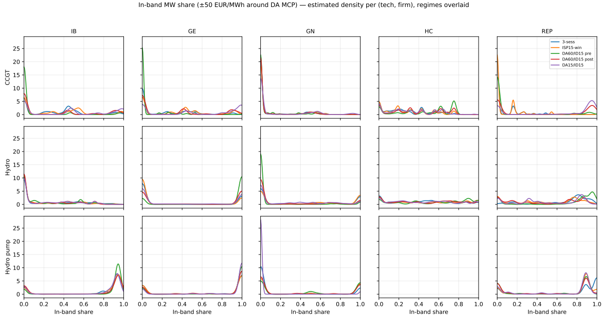
Figure 15: Estimated probability density of the daily in-band MW share per (tech, firm), regimes overlaid. Gaussian KDE across (unit, day, hour) cells per (firm, tech, regime). Bimodality visible for several CCGT firms under DA15/ID15 — mass clustered both near 0 (firm did not have MW close to MCP that day) and near 1 (firm fully in-band, often a single block at MCP). REP-CCGT under DA15/ID15 has clear bimodality with a large mass near 1, while GN-CCGT has most mass near 0. The reform-window shift to right tail is visible in the right-shifting curve across regimes for IB, GE, HC and REP CCGT.
