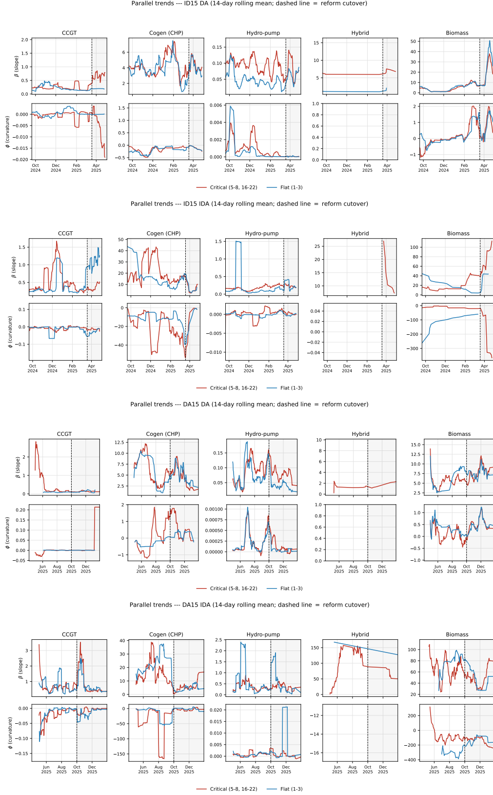
Figure 10: Pre-trends for \hat{\beta} and \hat{\phi} : drift. Same construction as Figure 9. These are within-curve OLS objects, mechanically sensitive to tranche counts and grid density — hence supporting, not headline.
