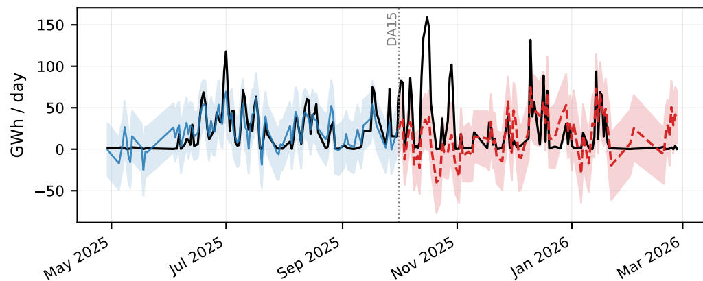
DA CCGT cleared
