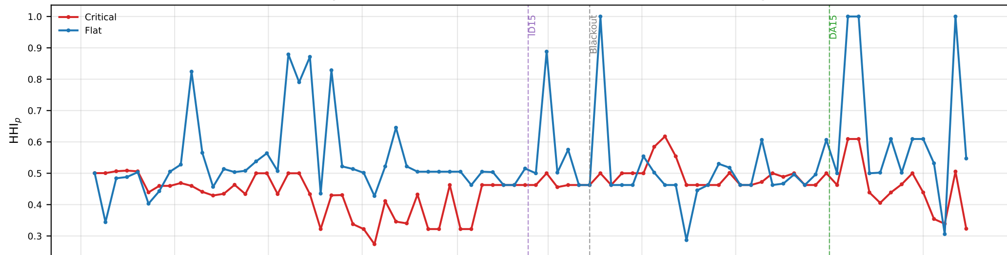
CCGT day-ahead per-curve hhi (critical = ramp hours, flat = overnight)
