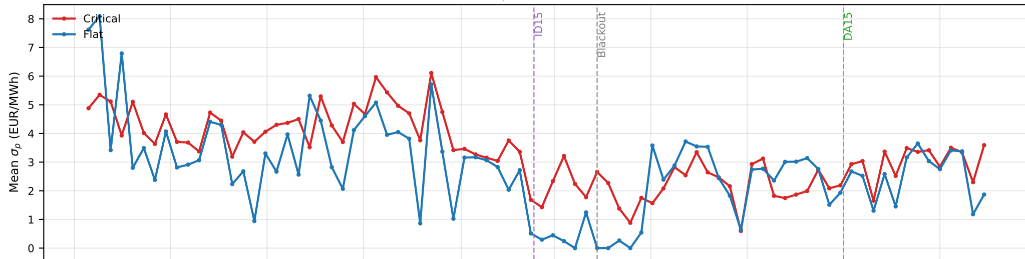
CCGT day-ahead within-quarter \sigma_p (critical = ramp hours, flat = overnight)
