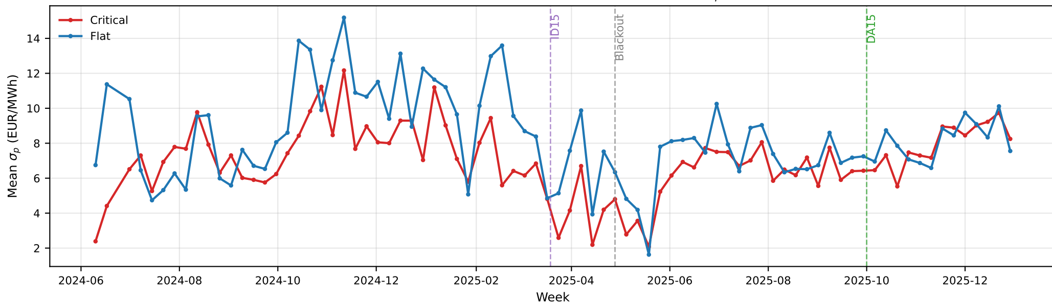
CCGT intraday-auction within-quarter \sigma_p
