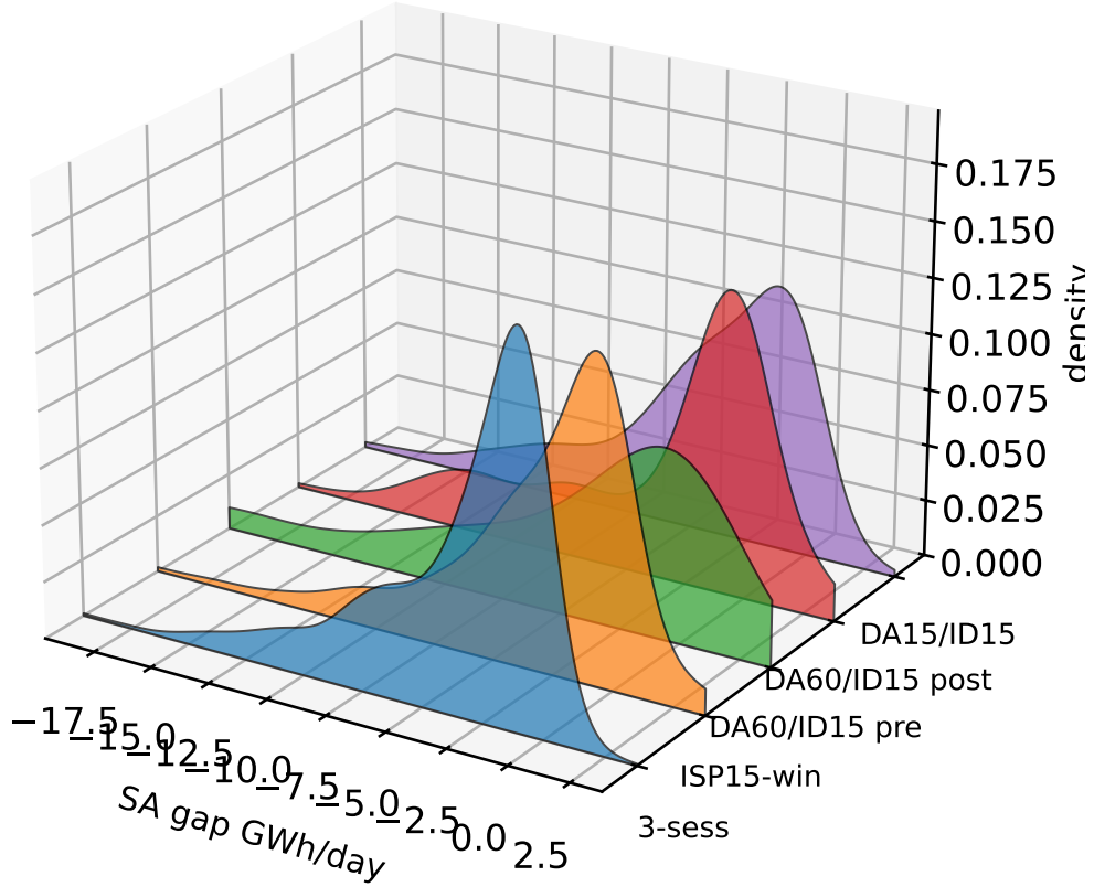
Figure 33: Hydro pump SA post-DA gap distribution, across regimes — 3D ridge. Companion to Fig. 32.
