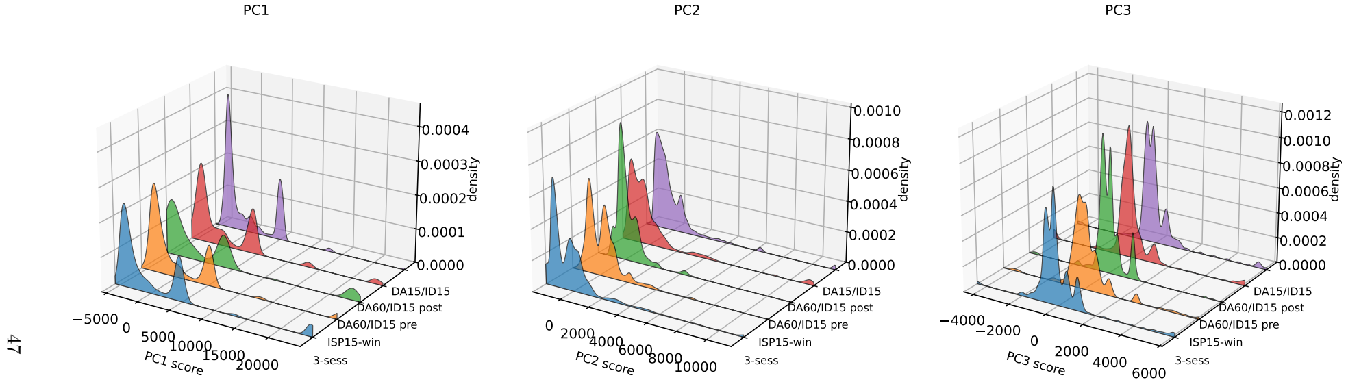
Figure 24: CCGT: distribution of functional-SA PC scores across regimes. Each panel is a 3D ridge plot of one principal component score; one curve per regime, stacked along the y -axis. Cell-level scores (per-(unit, day, period)) projected onto the per-tech aggregate basis; the basis itself is not shown (the per-unit decomposition in §3.4.1 is the maximum-granularity object). Bimodality emerges post-MTU15-IDA on PC1 and PC2.
