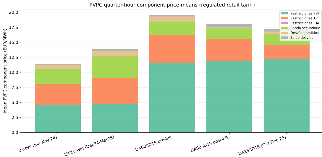
Figure 37: PVPC retail-tariff components, stacked. Total “restricciones técnicas” (PBF + TR + IDA) goes from €9.13/MWh (ISP15-win) to €14.56/MWh (DA15/ID15). The PBF (= Fase I) component drives the increase ( 4.7 \rightarrow 12.2 EUR/MWh, \sim \times 2.6 ); the TR component declines.
