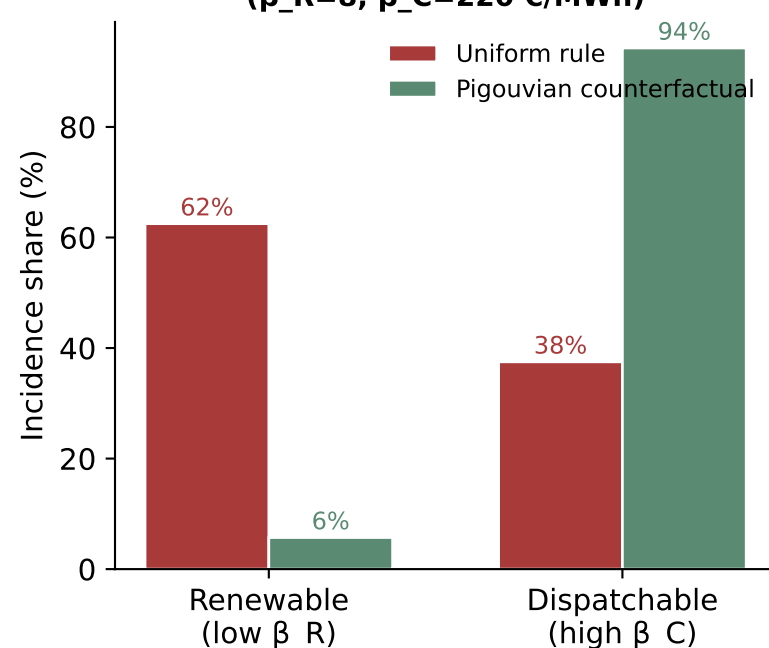
P5 — Pigouvian rule redistributes incidence weights ( \beta_R=8, \beta_C=220 \text{ €/MWh} )
