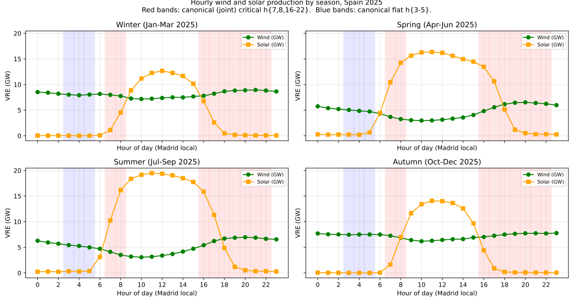
Figure 2: Hourly wind and solar production by season, Spain 2025. Four-panel decomposition by season. Red bands mark the canonical critical hours h \in \{7, 8, 16, 17, 18, 19, 20, 21, 22\} (the joint set: morning ramp \cup afternoon-evening peak). Blue bands mark the flat hours h \in \{3, 4, 5\} . Solar production is concentrated in midday hours and disappears in critical-hour bands; wind is broadly flat across the day with mild seasonality. The combination implies that critical hours systematically have low VRE supply year-round, supporting the use of the joint set as the strategically-relevant time-varying window.
