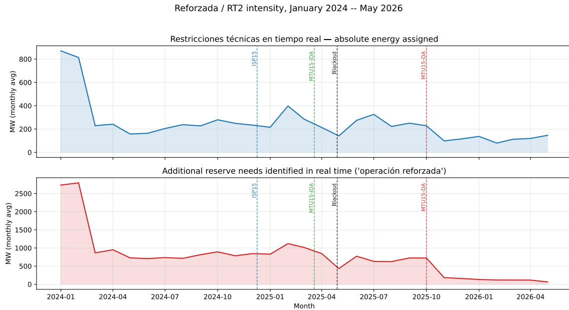
Figure 11: Reforzada / RT2 intensity, January 2024 – May 2026. Top panel: monthly average of absolute energy assigned via real-time technical restrictions (ESIOS indicator 10052). Bottom panel: monthly average of additional reserve needs identified in real time (ESIOS indicator 1880; coverage from 2021-05). Dashed vertical lines mark, in order, ISP15 (2024-12-09), MTU15-IDA (2025-03-19), the Iberian blackout (2025-04-28) and MTU15-DA (2025-10-01).
