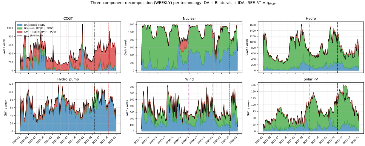
Figure 11: Weekly three-component decomposition of dispatch, by technology. PDBC (blue, day-ahead-cleared) + bilateral executions (green) + IDA + REE real-time top-up (red) = final post-IDA dispatch (black). Vertical guides: MTU15-IDA, April 2025 blackout, MTU15-DA.
