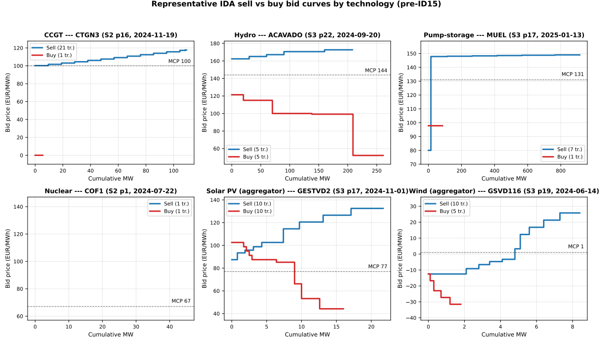
Figure 14: Representative IDA sell vs buy bid curves by technology, pre-ID15. One representative (unit, date, session, period) per tech. Blue: sell curve (supply, ascending in price). Red: buy curve (demand, descending in price). Dashed: MCP. Pre-ID15 window 2024-06-14 to 2025-03-18.
