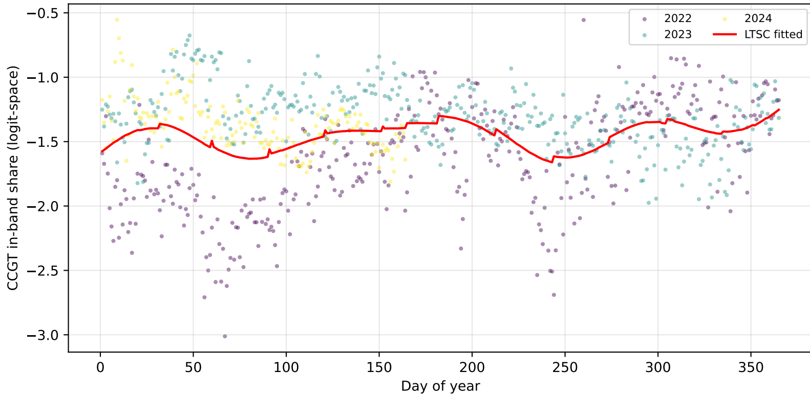
CCGT in-band share — pre-IDA seasonal cycle (yearly overlay)
