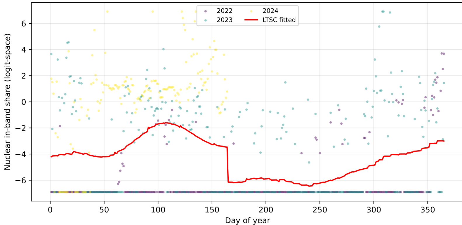
Nuclear in-band share — pre-IDA seasonal cycle (yearly overlay)
