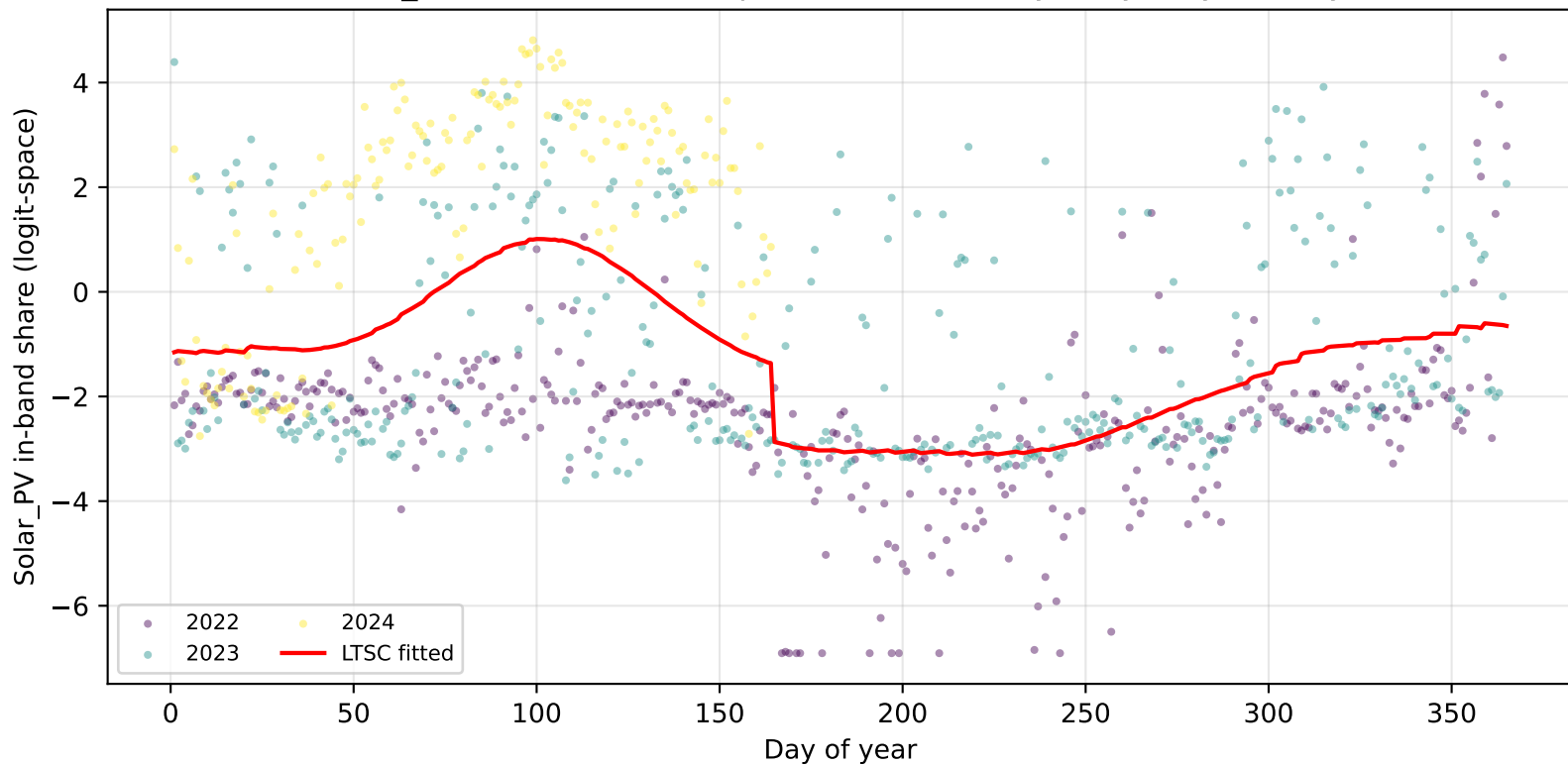
Solar_PV in-band share — pre-IDA seasonal cycle (yearly overlay)
