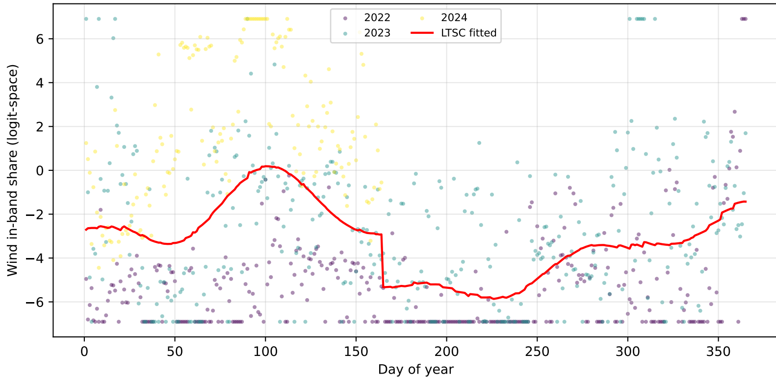
Wind in-band share — pre-IDA seasonal cycle (yearly overlay)
