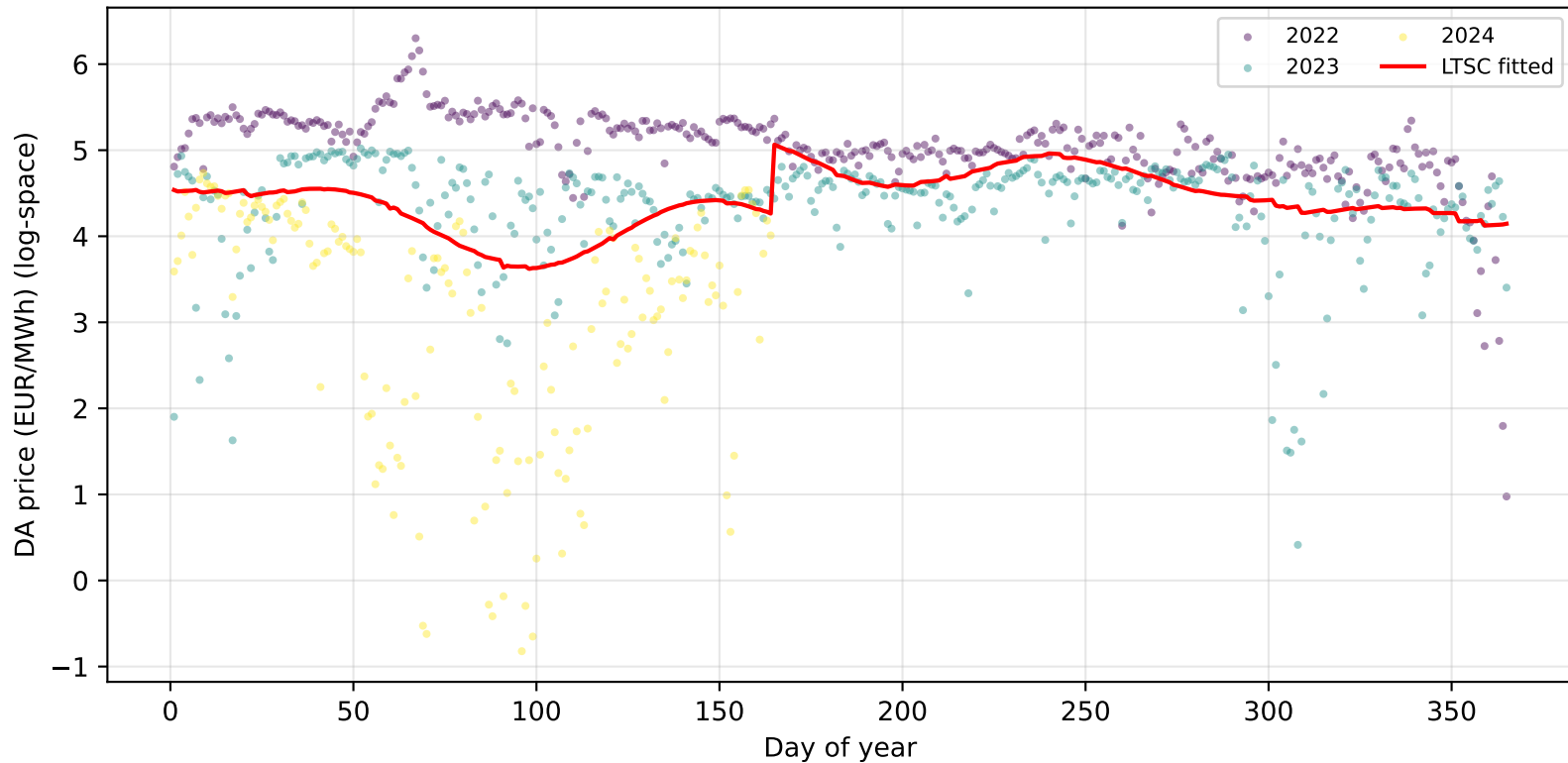
DA price (EUR/MWh) — pre-IDA seasonal cycle (yearly overlay)
