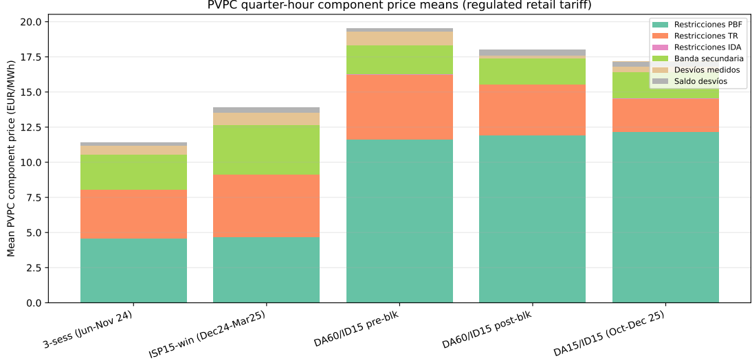
Figure 24: PVPC retail-tariff components, stacked. Total “restricciones técnicas” (PBF + TR + IDA) goes from €9.13/MWh (ISP15-win) to €14.56/MWh (DA15/ID15). The PBF (= Fase I) component drives the increase (4.7 → 12.2 EUR/MWh, \sim \times 2.6 ); the TR component declines.
