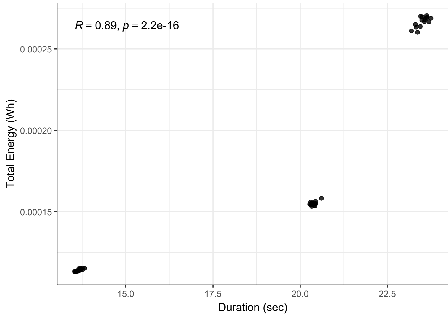
kroA100.tsp
