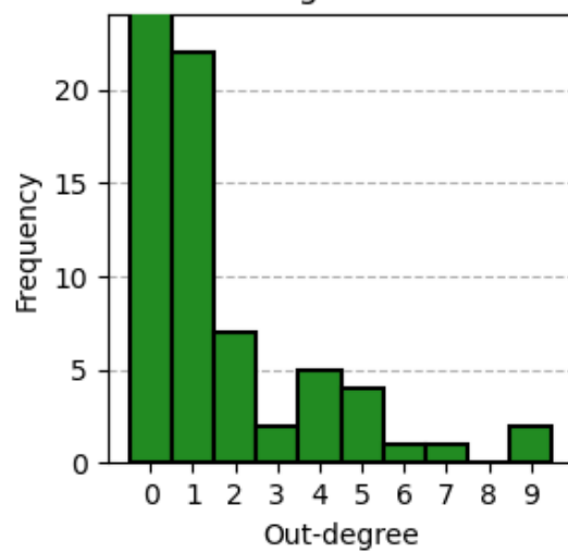
Out-degrees 51-84
