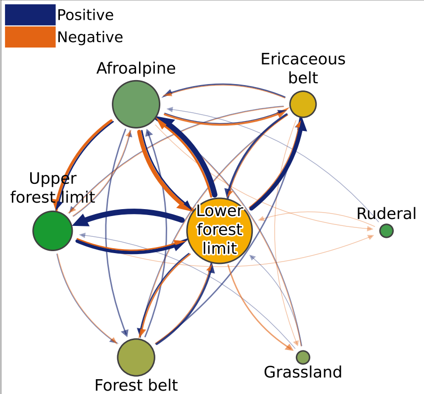
Period 4
