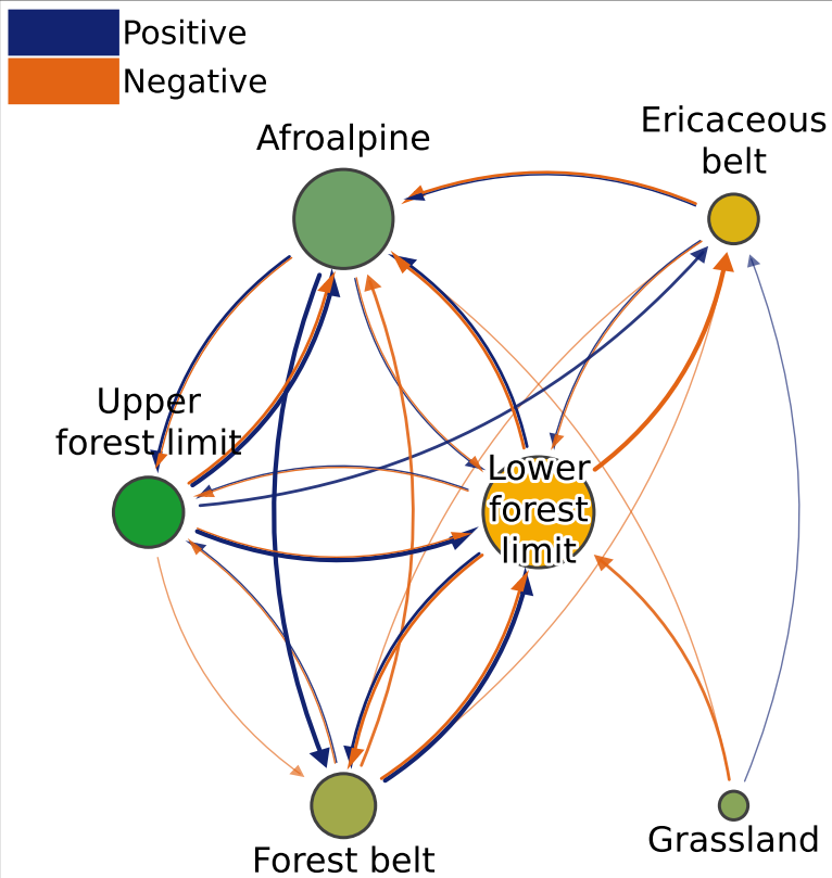
Period 3
