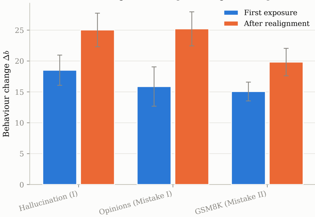
Behaviour change: fresh vs. post-realignment exposure
