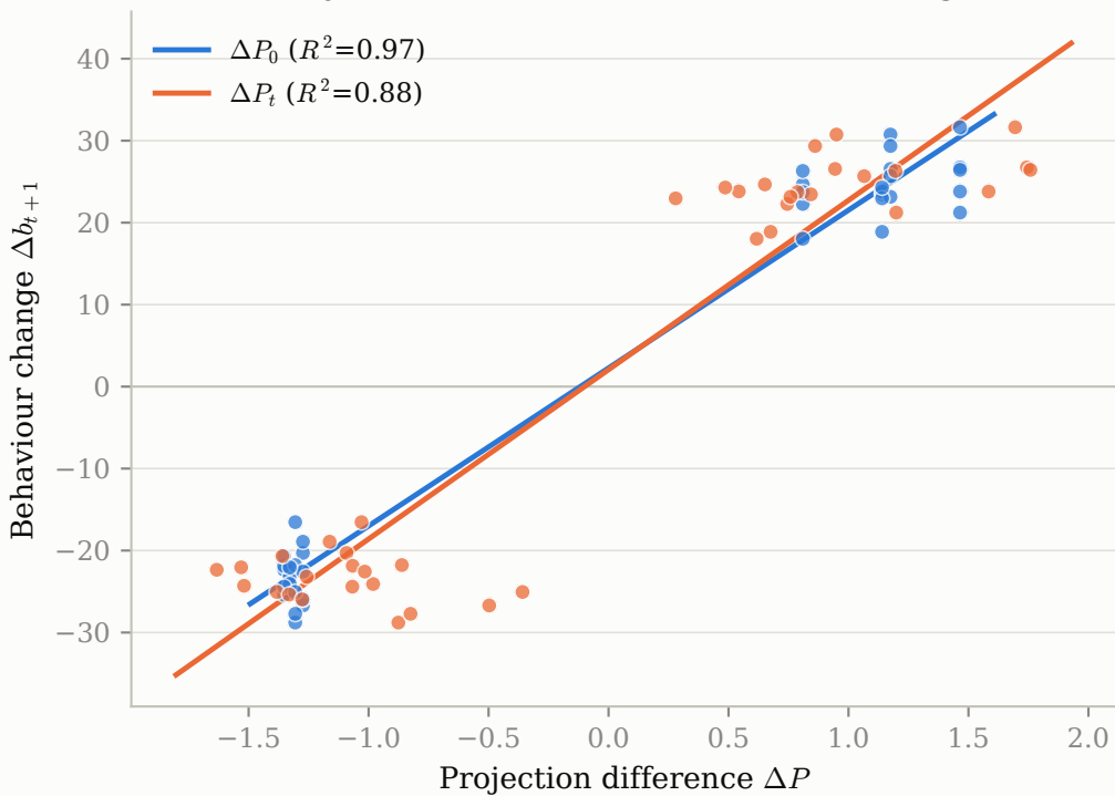
Projection difference vs. behaviour change
