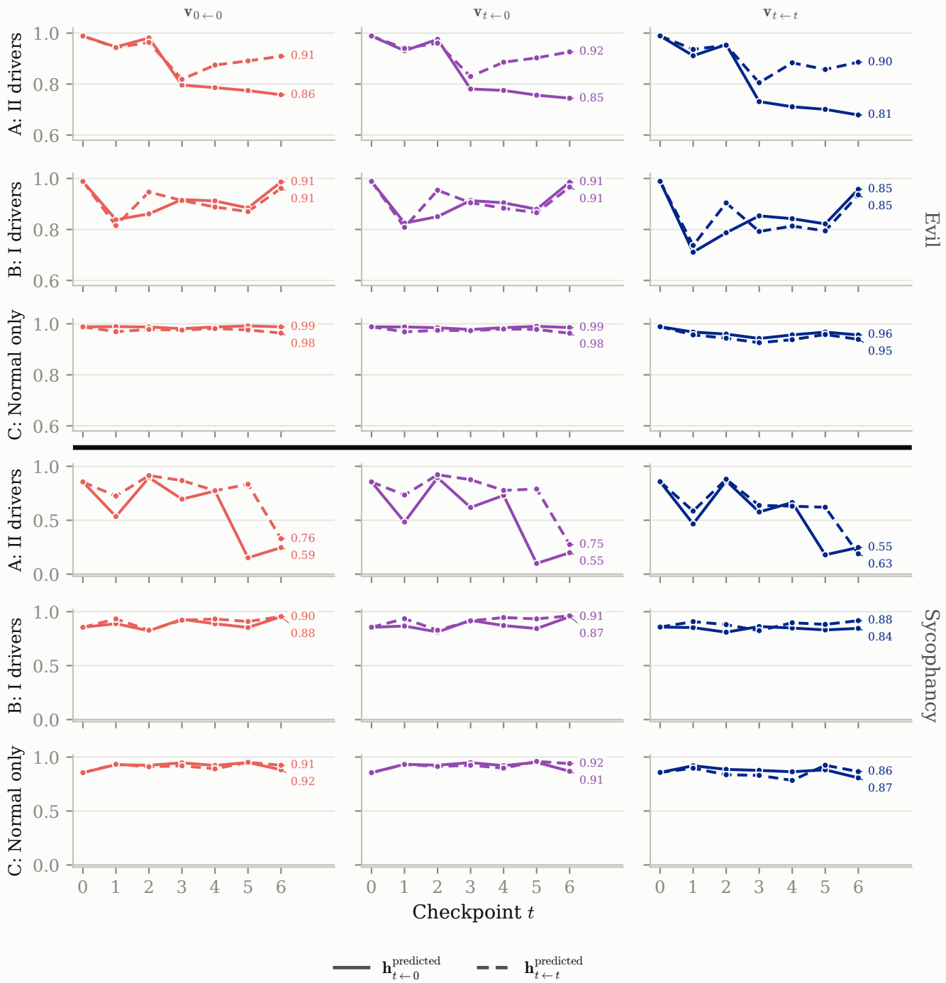
Correlation r with b_{t+1} over the probe set
