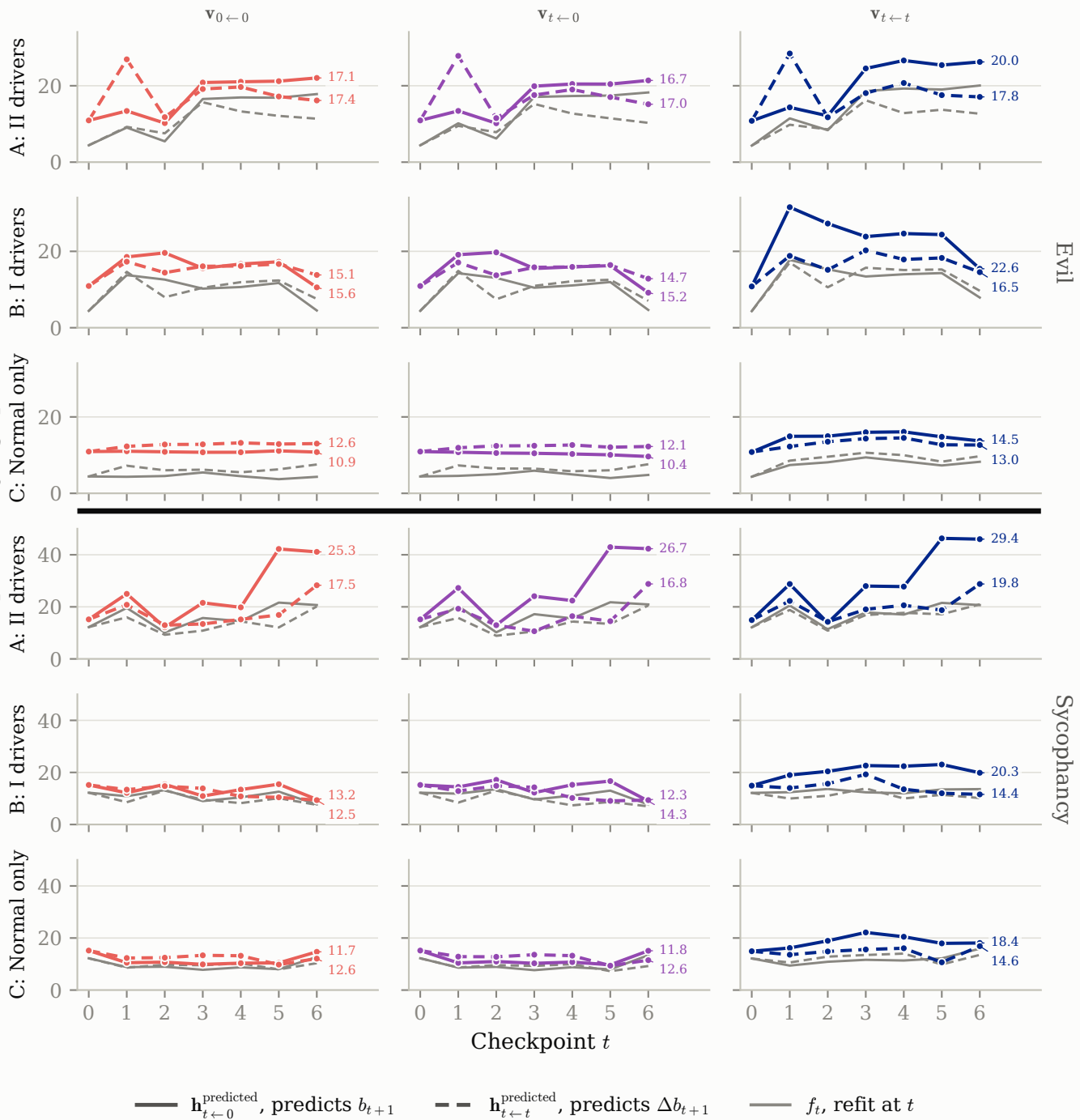
RMSE over the probe set (judge points)
