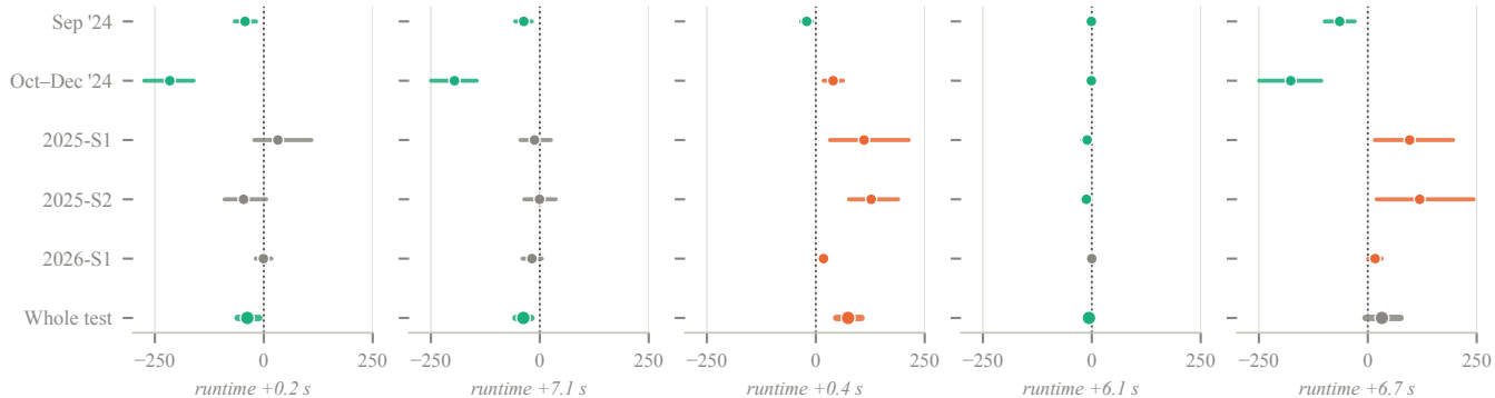
Online adaptation (ACI over static)
