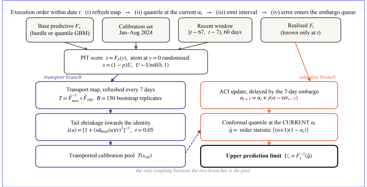
Figure 4: Data flow of the adaptive scheme, from the base predictive to the upper prediction limit. The transport branch (left) estimates and regularises the map; the adaptive branch (right) maintains the effective miscoverage level. The two are coupled only through the transported calibration pool, and the order of operations within a date is stated at the top: the conformal quantile is taken at the level in force before the day’s own error is observed, and that error is fed back only after the seven-day horizon embargo.
