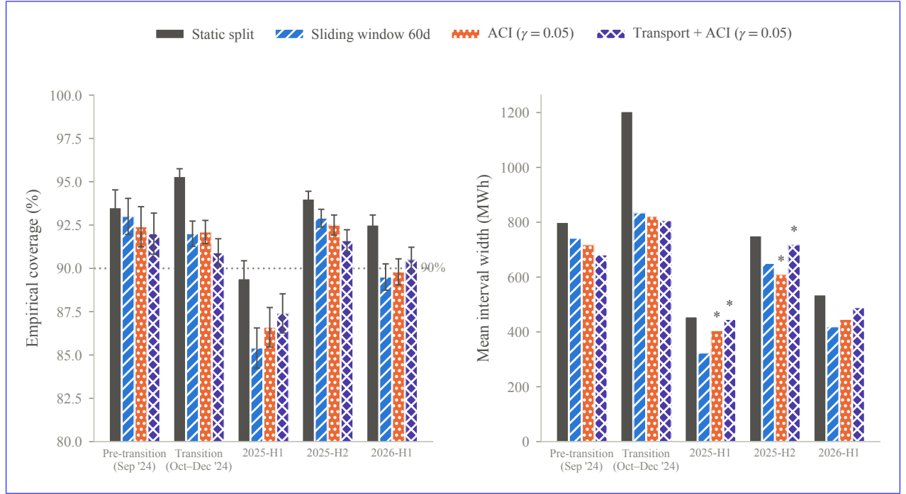
Figure 6: Coverage and sharpness by method and period, hurdle base model. Left: empirical coverage with date-clustered standard errors against the 90% nominal level. Right: mean interval width. Asterisks mark bars whose mean width is computed over finite intervals only, because the corresponding configuration returns at least 1% of infinite intervals.
