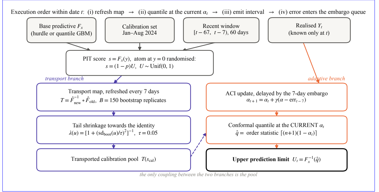
Figure 4: Data flow of the adaptive scheme, from the base predictive to the upper prediction limit. The transport branch (left) estimates and regularises the map; the adaptive branch (right) maintains the effective miscoverage level. The two are coupled only through the transported calibration pool, and the order of operations within a date is stated at the top: the conformal quantile is taken at the level in force before the day’s own error is observed, and that error is fed back only after the seven-day horizon embargo.
