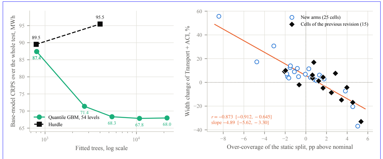
Figure 8: Left: base-model CRPS over the whole test against the number of fitted trees, at a fixed 54-level quantile grid for the multi-quantile predictive. The hurdle is shown at its own budget and at five times it. Right: the diagnostic relationship over the forty cells, with the fifteen cells of the previous revision marked separately, the fitted line over all forty, and its bootstrap interval. The new arms populate the region below nominal coverage, where the previous design had no point.
