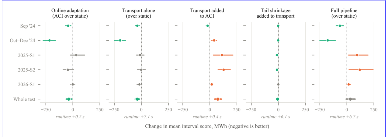
Figure 9: Marginal contribution of each component of the adaptive scheme to the mean interval score, by window, with 95% bootstrap intervals resampling whole days. Green marks a significant improvement, orange a significant deterioration, grey an interval containing zero. Runtime is the additional wall-clock cost of each component.
