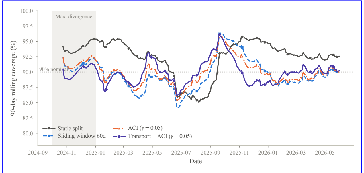
Figure 5: Rolling empirical coverage (90-day window) of the conformal methods on real data with the hurdle base model, computed with the 7-day horizon embargo. The dashed line marks the 90% nominal level and the shaded band marks the window of maximum divergence from the calibration distribution, October to December 2024. The static split drifts into over-coverage as that window advances, whereas the adaptive schemes remain close to nominal.
