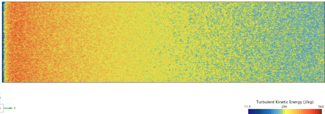
Ribbed case turbulent kinetic energy
