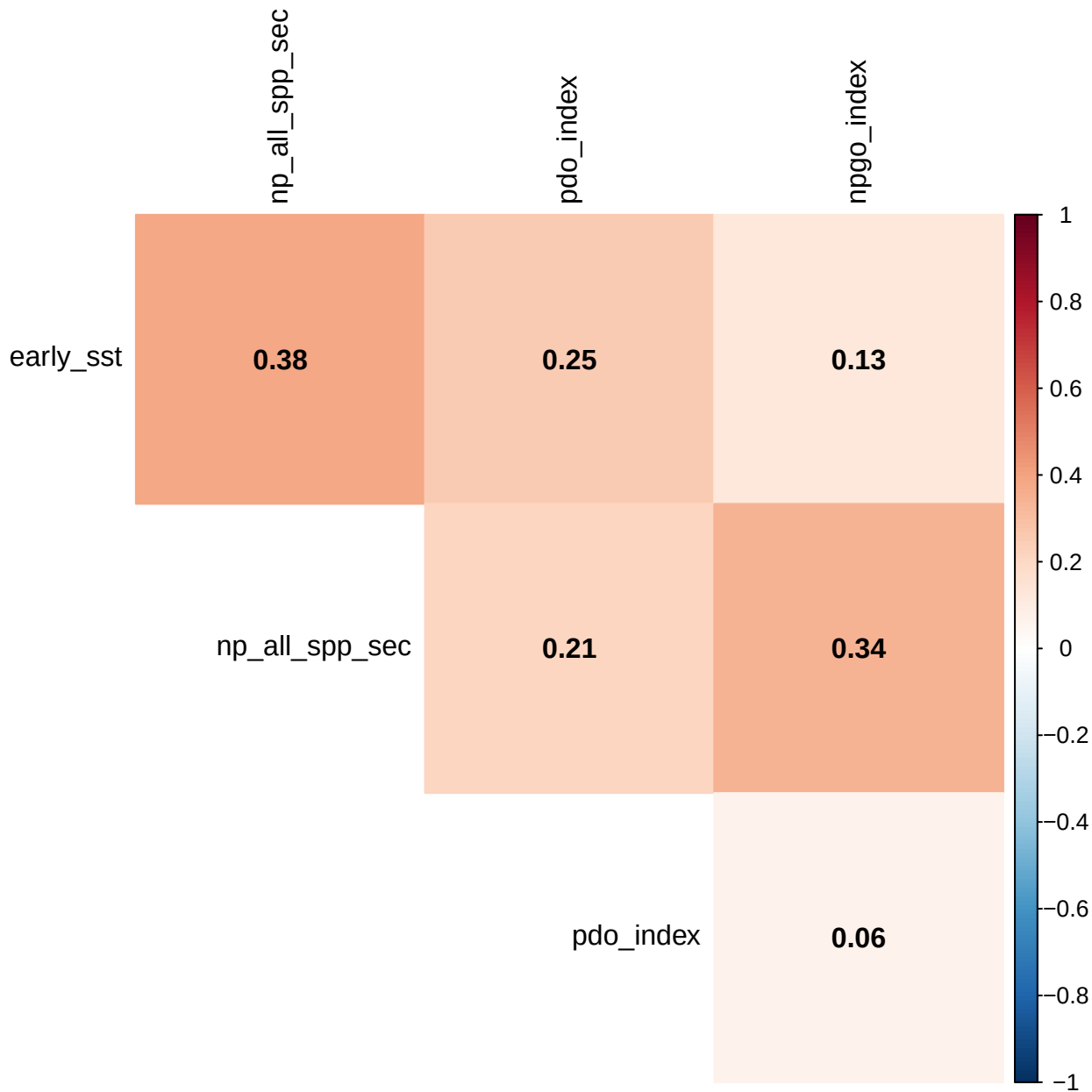
Average stock-specific covariate correlations 1950 – 1988
