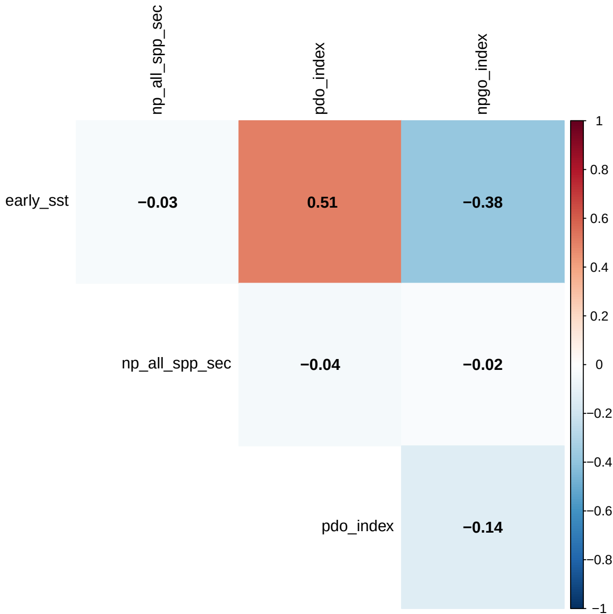
Average stock-specific covariate correlations 1989 – 2010
