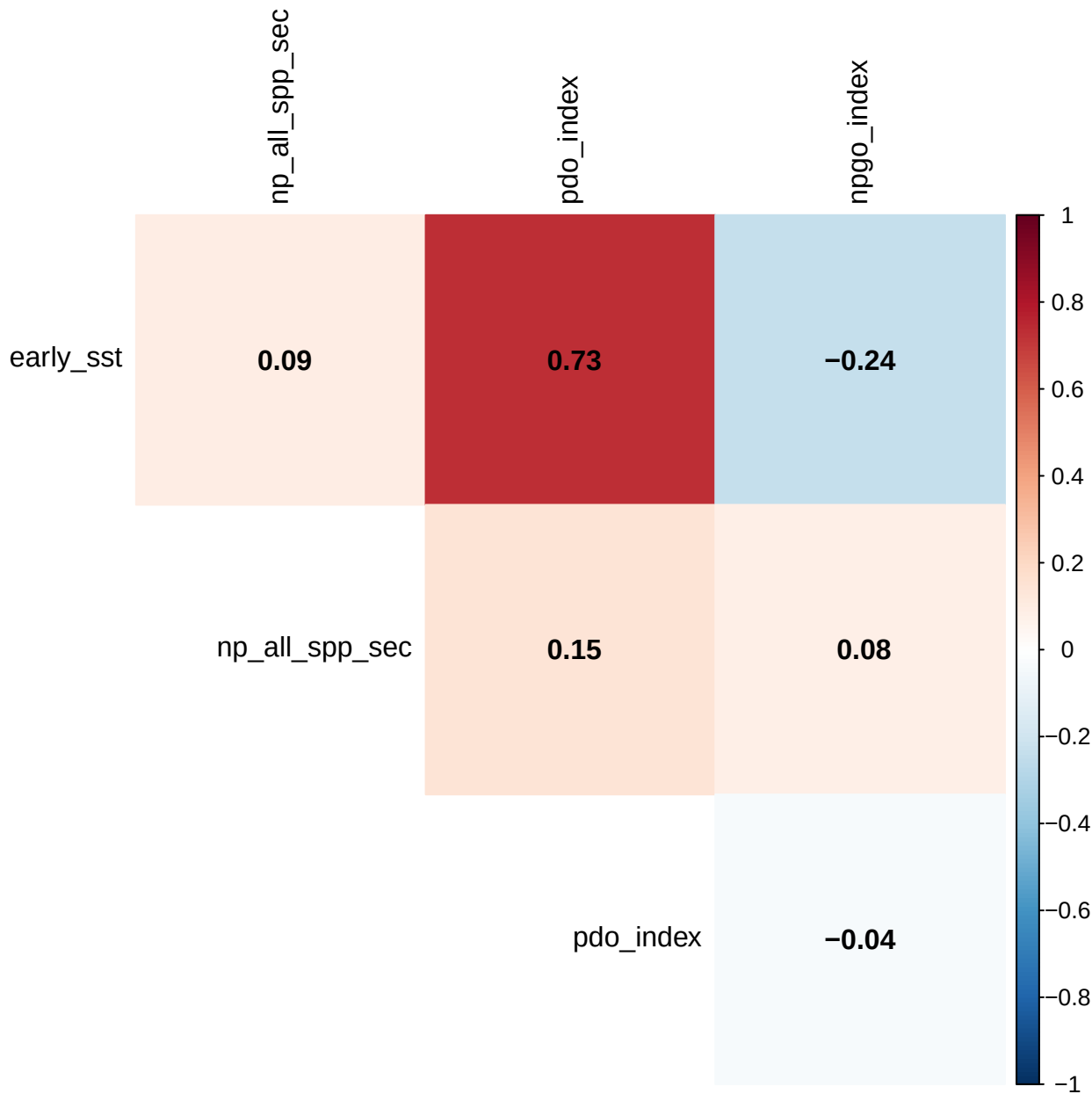
Average stock-specific covariate correlations 2011 – 2019
