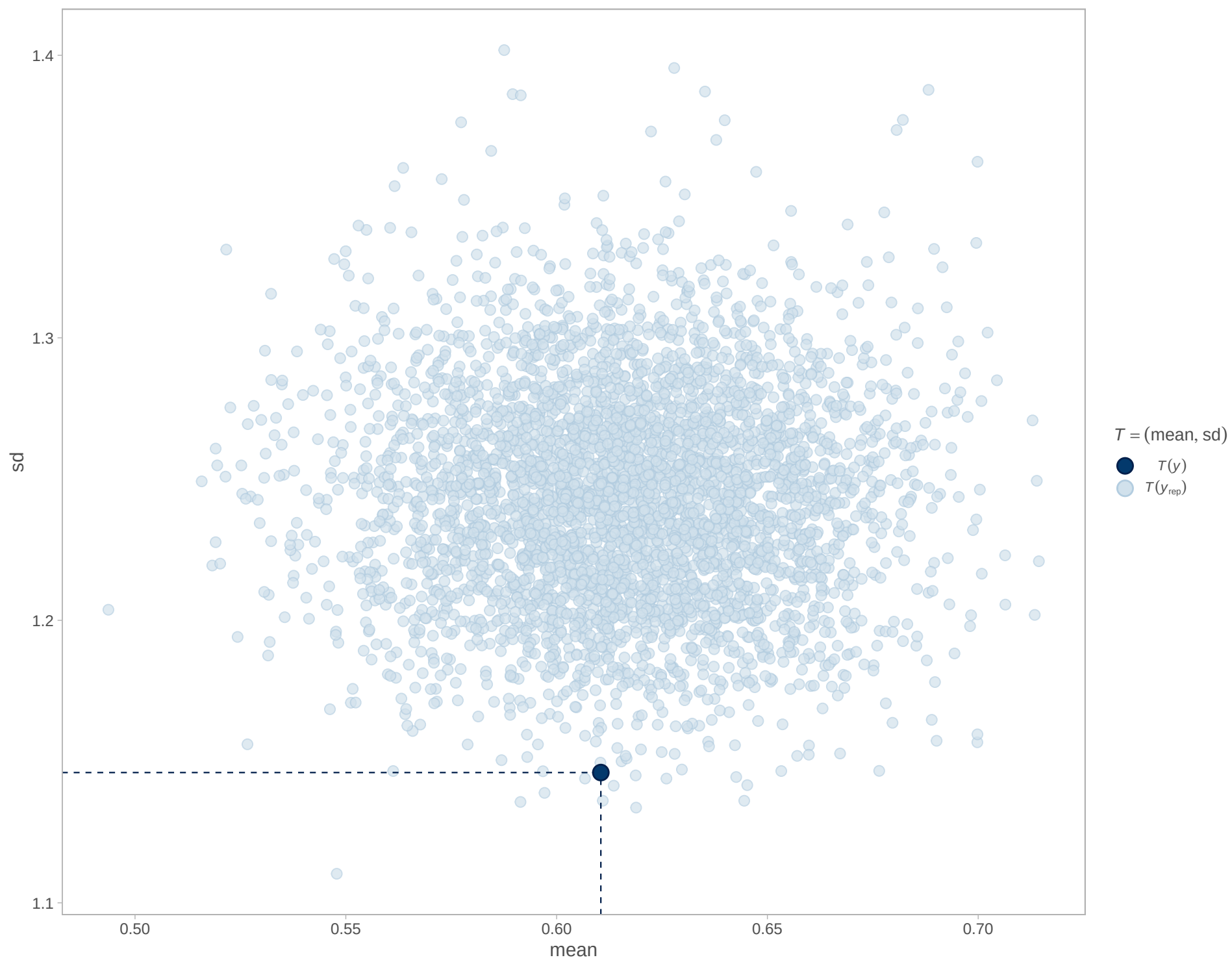
Y rep: target distributions
