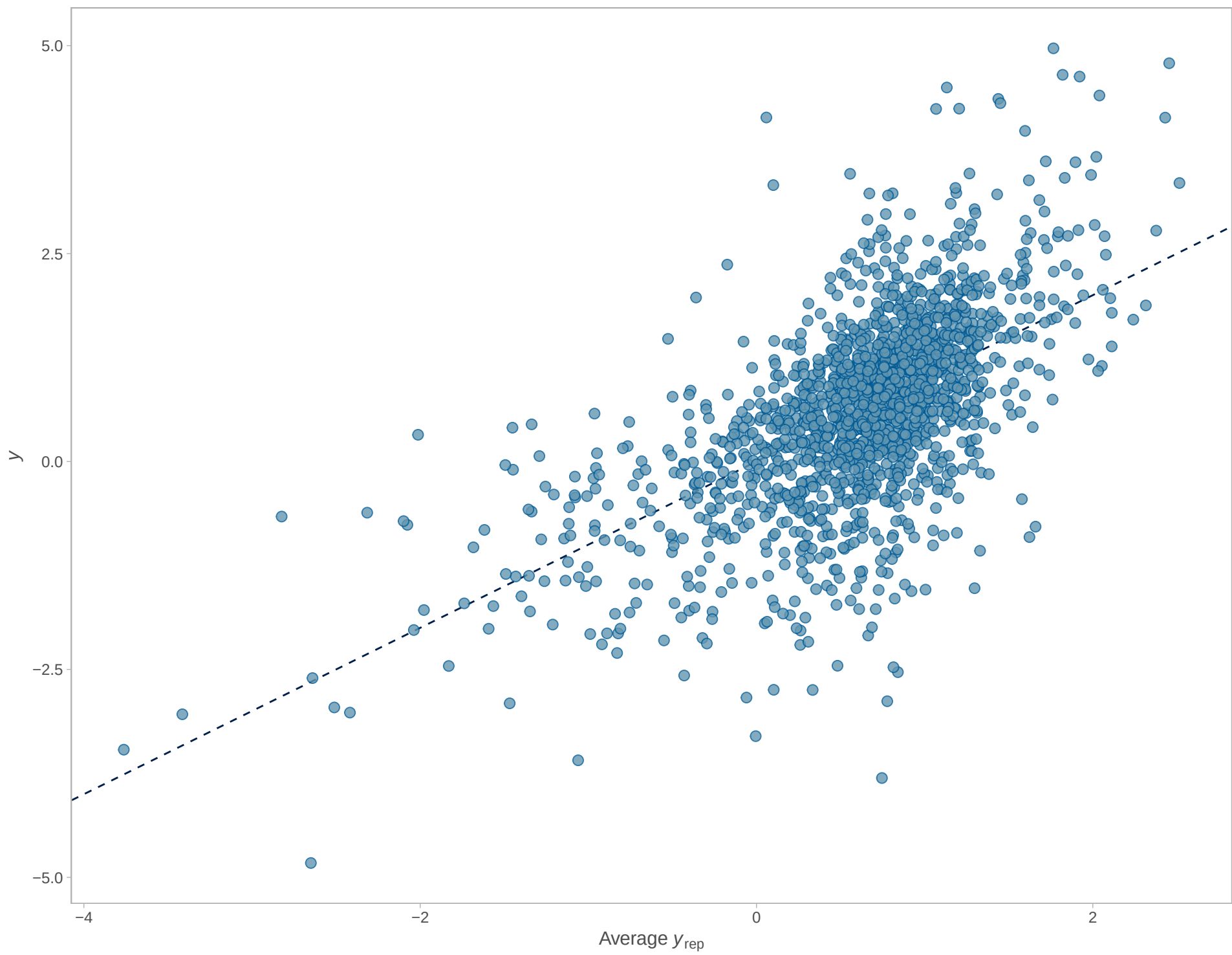
Observed vs. predicted
