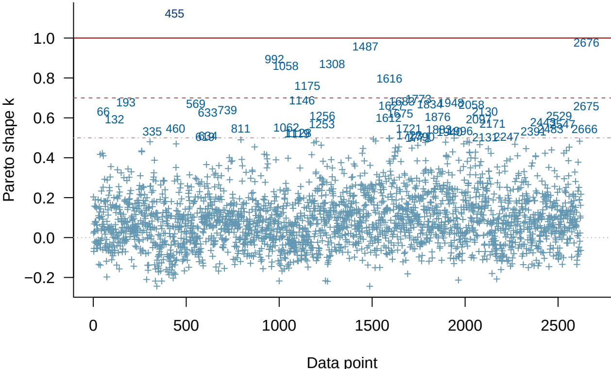
PSIS diagnostic plot
